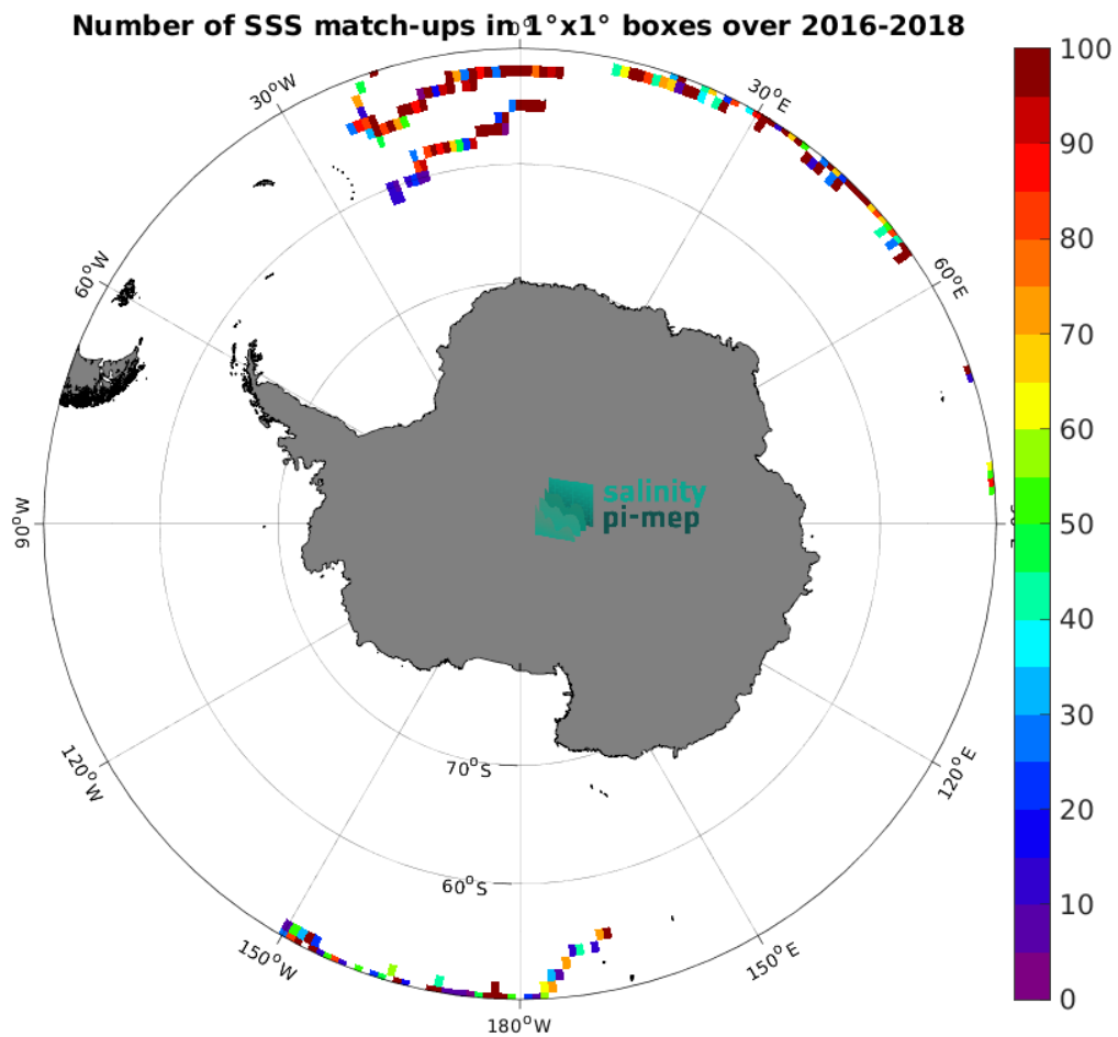
Figure 4: Number of SSS match-ups between Surface drifters SSS and the SMOS SSS L3 v335 - 10 Days - 25 km (CATDS-CPDC) SSS product for the Southern Ocean Pi-MEP region over 1^\circ \times 1^\circ boxes and for the full satellite product period.
