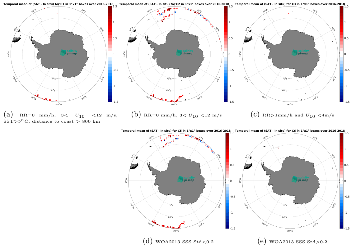
Figure 13: Temporal mean gridded over spatial boxes of size 1^\circ \times 1^\circ of \Delta\text{SSS} (SMOS SSS L3 v335 - 10 Days - 25 km (CATDS-CPDC) - Surface drifters) for 5 different subdatasets corresponding to: RR=0 mm/h, 3 < U_{10} < 12 m/s, SST >5^\circ\text{C} , distance to coast > 800 km (a), RR=0 mm/h, 3 < U_{10} < 12 m/s (b), RR >1 mm/h and U_{10} < 4 m/s (c), WOA2013 SSS Std <0.2 (d), WOA2013 SSS Std >0.2 (e).
