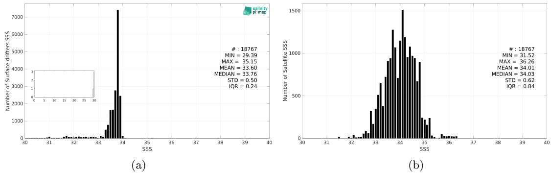
Figure 3: Histograms of SSS from Surface drifters (a) and SMOS SSS L3 v335 - 10 Days - 25 km (CATDS-CPDC) (b) considering all match-up pairs per bins of 0.1 over the Southern Ocean Pi-MEP region and for the full satellite product period.
