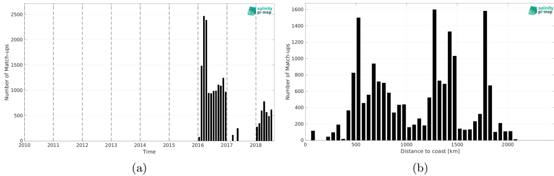
Figure 2: Number of match-ups between Surface drifters and SMOS SSS L3 v335 - 10 Days - 25 km (CATDS-CPDC) SSS as a function of time (a) and as function of the distance to coast (b) over the Southern Ocean Pi-MEP region and for the full satellite product period.
