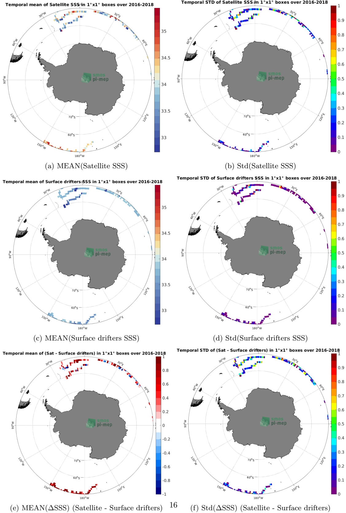
Figure 5: Temporal mean (left) and Std (right) of SSS from SMOS SSS L3 v335 - 10 Days - 25 km (CATDS-CPDC) (top), Surface drifters (middle), and of \Delta SSS (Satellite - Surface drifters). Only match-up pairs are used to generate these maps.
