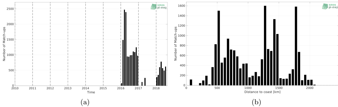
Figure 1: Number of match-ups between Surface drifters and SMOS SSS L3 v335 - 10 Days - 25 km (CATDS-CPDC) SSS as a function of time (a) and as function of the distance to coast (b) over the Southern Ocean Pi-MEP region and for the full satellite product period.
