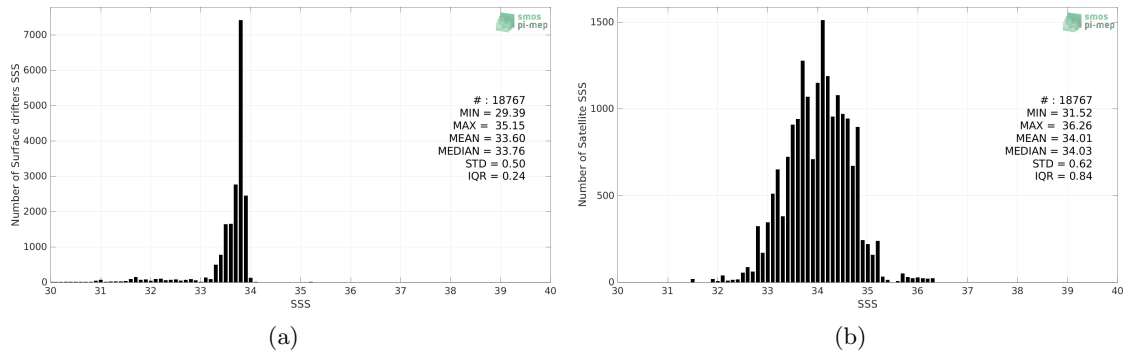
Figure 2: Histograms of SSS from Surface drifters (a) and SMOS SSS L3 v335 - 10 Days - 25 km (CATDS-CPDC) (b) considering all match-up pairs per bins of 0.1 over the Southern Ocean Pi-MEP region and for the full satellite product period.
