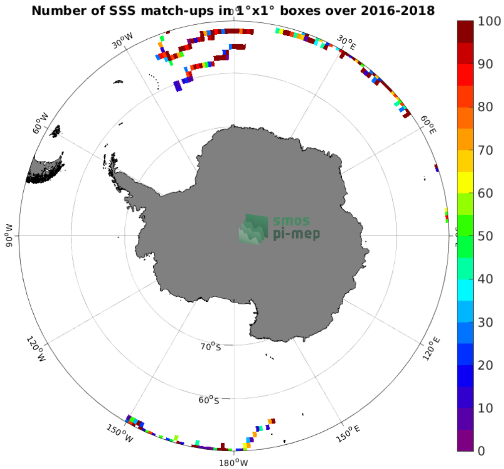
Figure 3: Number of SSS match-ups between Surface drifters SSS and the SMOS SSS L3 v335 - 10 Days - 25 km (CATDS-CPDC) SSS product for the Southern Ocean Pi-MEP region over 1^\circ \times 1^\circ boxes and for the full satellite product period.
