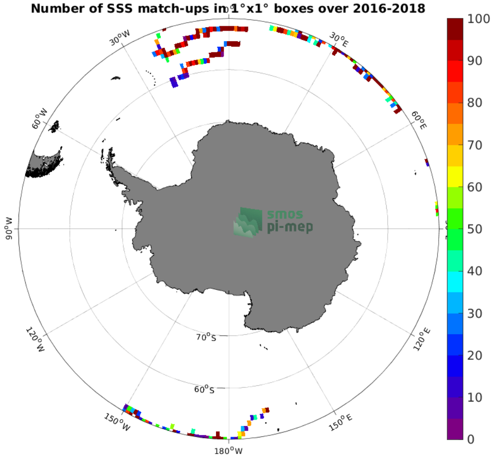
Figure 3: Number of SSS match-ups between Surface drifters SSS and the SMOS SSS L3 v335 - 10 Days - 25 km (CATDS-CPDC) SSS product for the Southern Ocean Pi-MEP region over 1^\circ \times 1^\circ boxes and for the full satellite product period.
