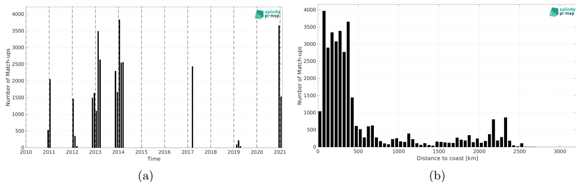
Figure 2: Number of match-ups between TSG (GOSUD-Sailing-ship) and SMOS SSS L2Q v333 - 0.25 Deg (CATDS-CPDC) SSS as a function of time (a) and as function of the distance to coast (b) over the Southern Ocean Pi-MEP region and for the full satellite product period.
