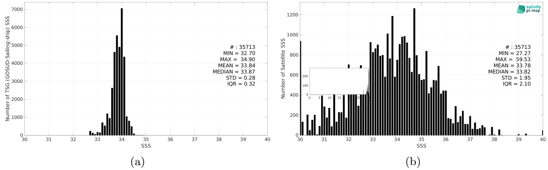
Figure 3: Histograms of SSS from TSG (GOSUD-Sailing-ship) (a) and SMOS SSS L2Q v333 - 0.25 Deg (CATDS-CPDC) (b) considering all match-up pairs per bins of 0.1 over the Southern Ocean Pi-MEP region and for the full satellite product period.
