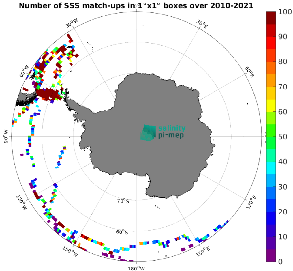
Figure 5: Number of SSS match-ups between TSG (GOSUD-Sailing-ship) SSS and the SMOS SSS L2Q v333 - 0.25 Deg (CATDS-CPDC) SSS product for the Southern Ocean Pi-MEP region over 1^\circ \times 1^\circ boxes and for the full satellite product period.
