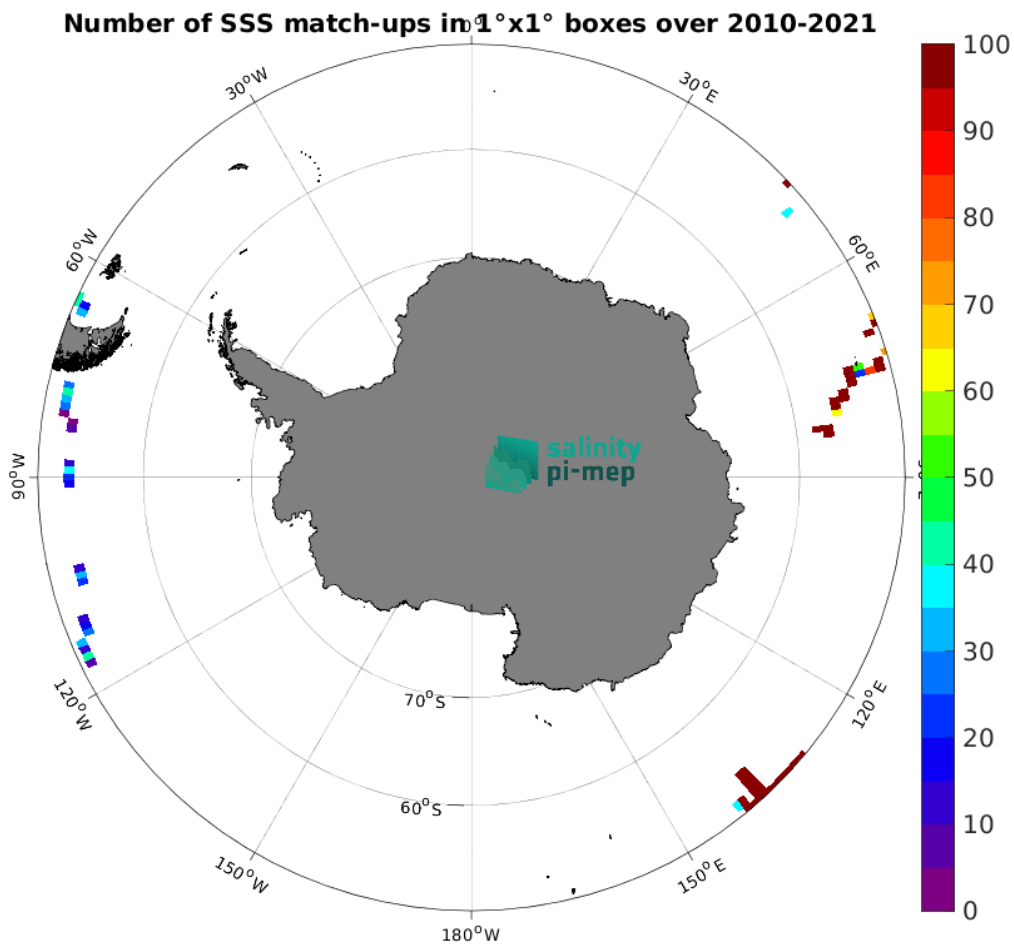
Figure 5: Number of SSS match-ups between TSG (GOSUD-Research-vessel) SSS and the SMOS SSS L2Q v333 - 0.25 Deg (CATDS-CPDC) SSS product for the Southern Ocean Pi-MEP region over 1^{\circ} \times 1^{\circ} boxes and for the full satellite product period.
