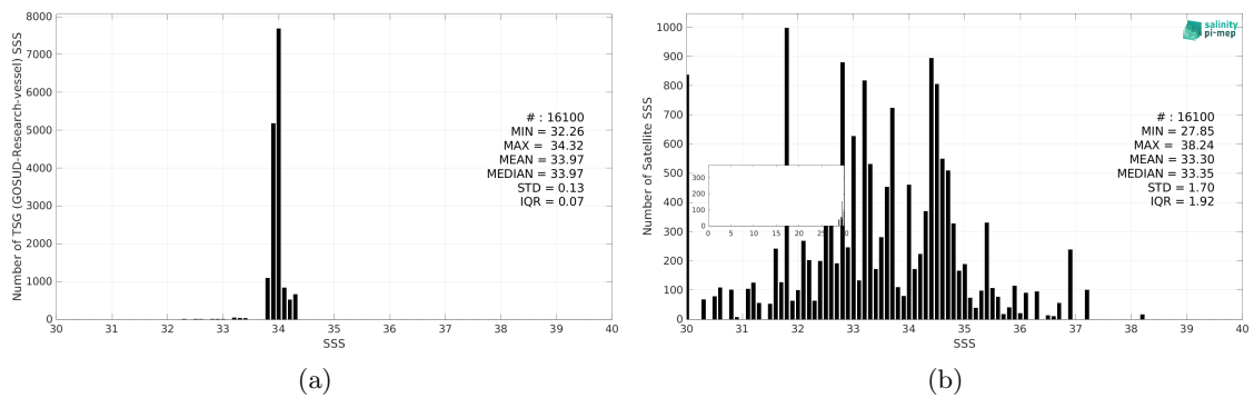
Figure 3: Histograms of SSS from TSG (GOSUD-Research-vessel) (a) and SMOS SSS L2Q v333 - 0.25 Deg (CATDS-CPDC) (b) considering all match-up pairs per bins of 0.1 over the Southern Ocean Pi-MEP region and for the full satellite product period.
