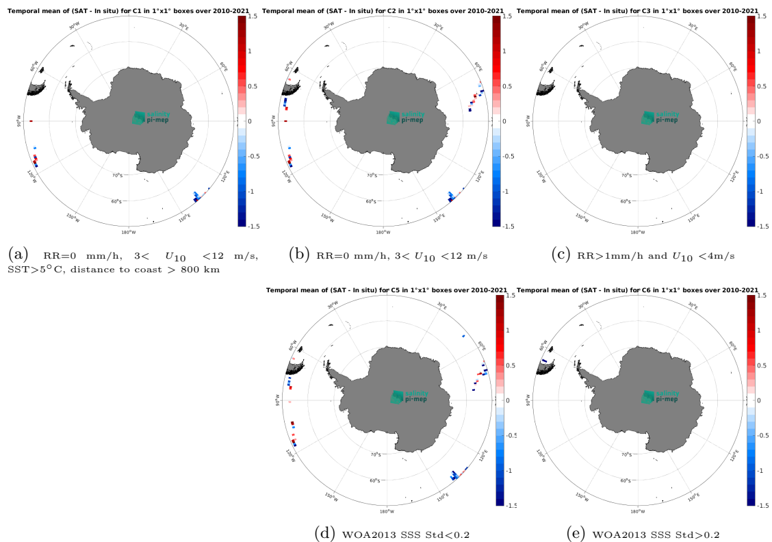
Figure 14: Temporal mean gridded over spatial boxes of size 1^\circ \times 1^\circ of \Delta\text{SSS} (SMOS SSS L2Q v333 - 0.25 Deg (CATDS-CPDC) - TSG (GOSUD-Research-vessel)) for 5 different subdatasets corresponding to:RR=0 mm/h, 3 < U_{10} < 12 m/s, SST>5°C, distance to coast > 800 km (a), RR=0 mm/h, 3 < U_{10} < 12 m/s (b), RR>1mm/h and U_{10} < 4 m/s (c), WOA2013 SSS Std<0.2 (d), WOA2013 SSS Std>0.2 (e).
