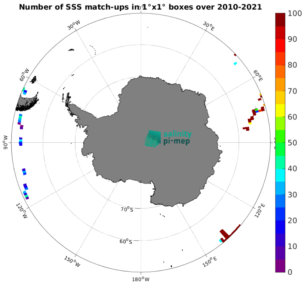
Figure 5: Number of SSS match-ups between TSG (GOSUD-Research-vessel) SSS and the SMOS SSS L2Q v333 - 0.25 Deg (CATDS-CPDC) SSS product for the Southern Ocean Pi-MEP region over 1^\circ \times 1^\circ boxes and for the full satellite product period.
