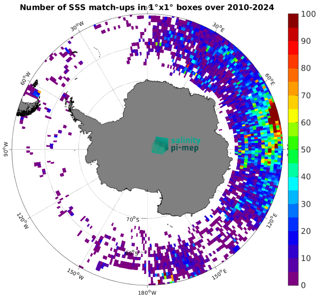
Figure 5: Number of SSS match-ups between Marine mammals SSS and the SMOS SSS L2Q v333 - 0.25 Deg (CATDS-CPDC) SSS product for the Southern Ocean Pi-MEP region over 1^\circ \times 1^\circ boxes and for the full satellite product period.
