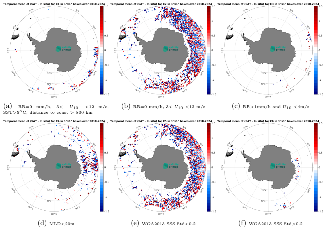
Figure 14: Temporal mean gridded over spatial boxes of size 1^\circ \times 1^\circ of \Delta SSS (SMOS SSS L2Q v333 - 0.25 Deg (CATDS-CPDC) - Marine mammals) for 6 different subdatasets corresponding to:RR=0 mm/h, 3 < U_{10} < 12 m/s, SST>5°C, distance to coast > 800 km (a), RR=0 mm/h, 3 < U_{10} < 12 m/s (b), RR>1mm/h and U_{10} < 4 m/s (c),MLD<20m (d),WOA2013 SSS Std<0.2 (e),WOA2013 SSS Std>0.2 (f).
