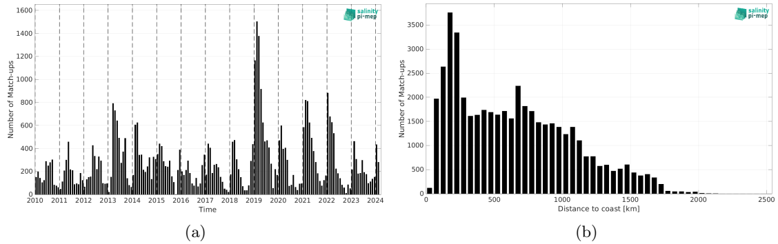
Figure 2: Number of match-ups between Marine mammals and SMOS SSS L2Q v333 - 0.25 Deg (CATDS-CPDC) SSS as a function of time (a) and as function of the distance to coast (b) over the Southern Ocean Pi-MEP region and for the full satellite product period.
