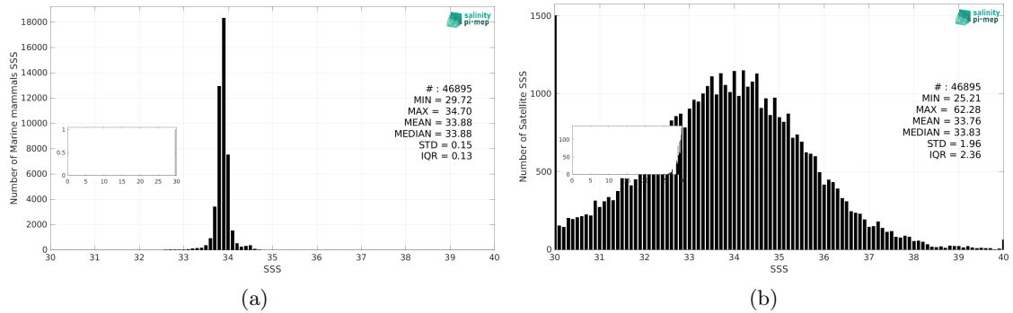
Figure 3: Histograms of SSS from Marine mammals (a) and SMOS SSS L2Q v333 - 0.25 Deg (CATDS-CPDC) (b) considering all match-up pairs per bins of 0.1 over the Southern Ocean Pi-MEP region and for the full satellite product period.
