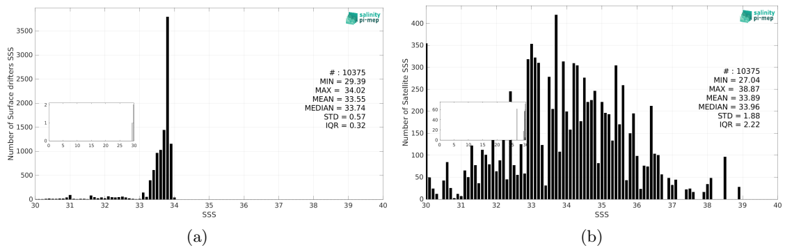
Figure 3: Histograms of SSS from Surface drifters (a) and SMOS SSS L2Q v333 - 0.25 Deg (CATDS-CPDC) (b) considering all match-up pairs per bins of 0.1 over the Southern Ocean Pi-MEP region and for the full satellite product period.
