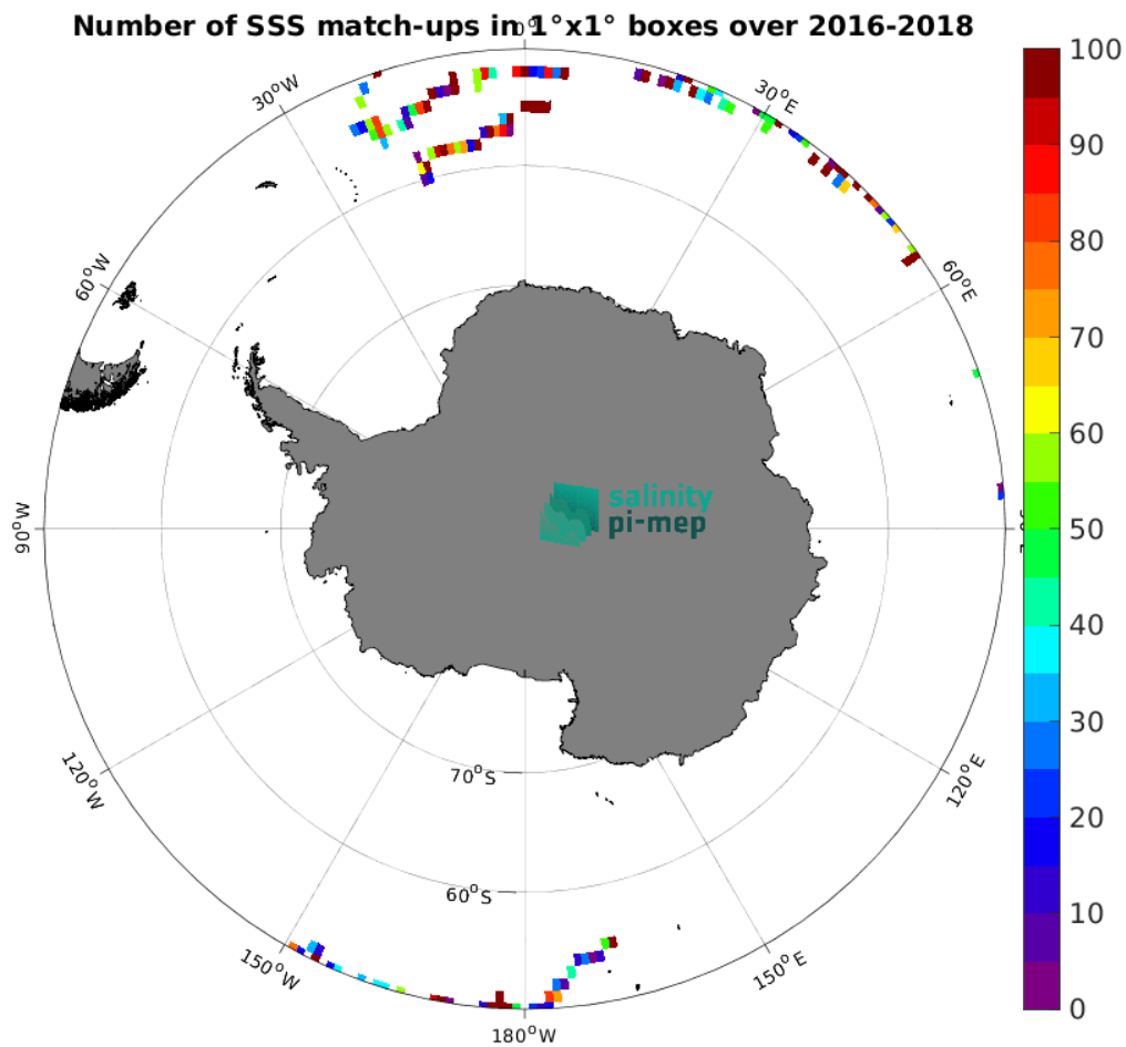
Figure 4: Number of SSS match-ups between Surface drifters SSS and the SMOS SSS L2Q v333 - 0.25 Deg (CATDS-CPDC) SSS product for the Southern Ocean Pi-MEP region over 1^{\circ} \times 1^{\circ} boxes and for the full satellite product period.
