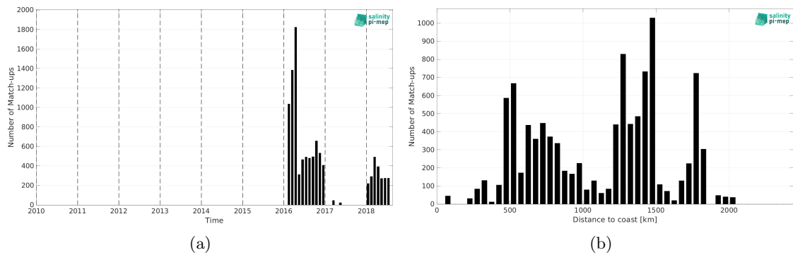
Figure 2: Number of match-ups between Surface drifters and SMOS SSS L2Q v333 - 0.25 Deg (CATDS-CPDC) SSS as a function of time (a) and as function of the distance to coast (b) over the Southern Ocean Pi-MEP region and for the full satellite product period.
