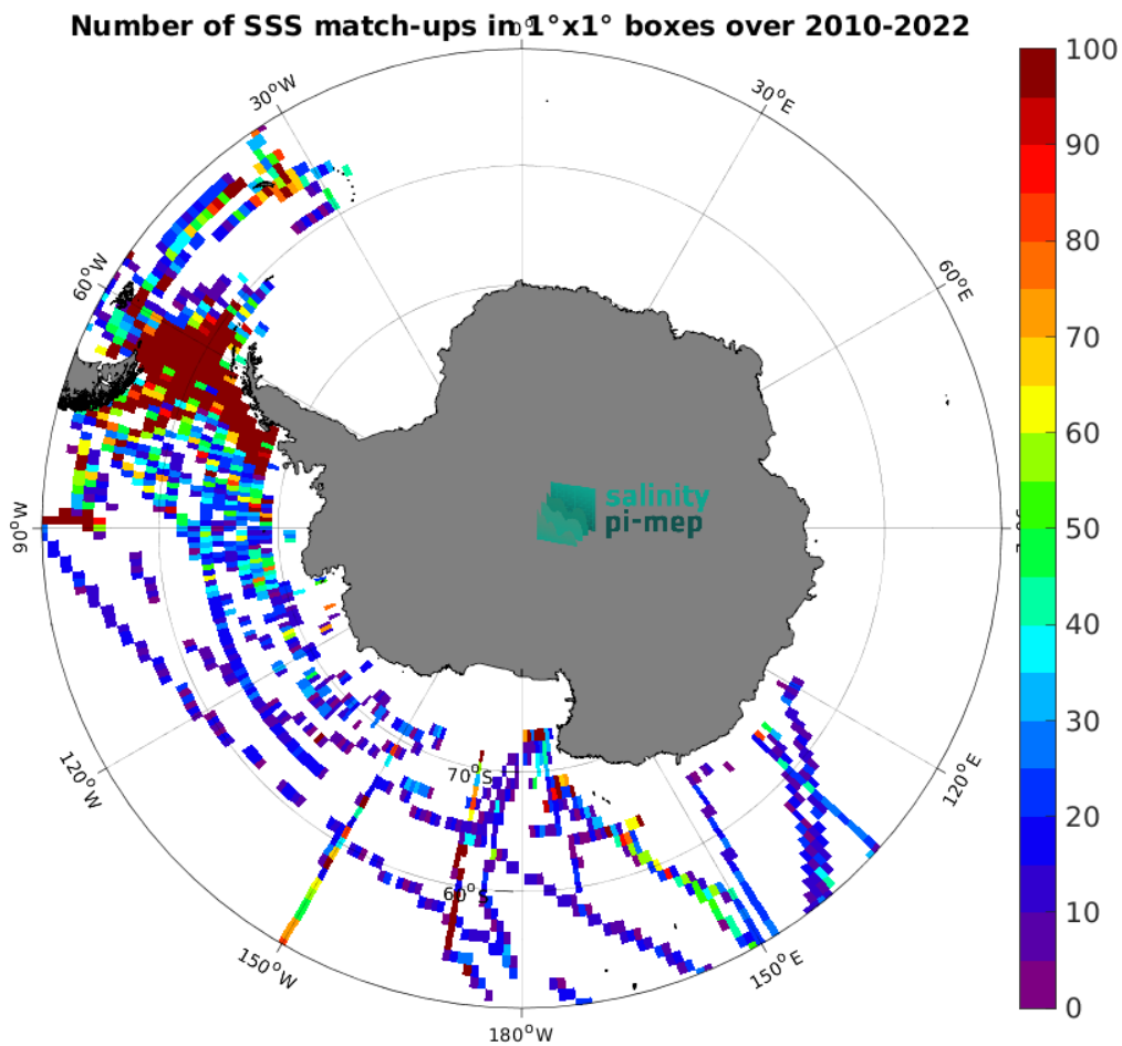
Figure 5: Number of SSS match-ups between TSG (SAMOS) SSS and the SMOS SSS L3 v332 - 9 Days (CATDS-CPDC) SSS product for the Southern Ocean Pi-MEP region over 1^\circ \times 1^\circ boxes and for the full satellite product period.
