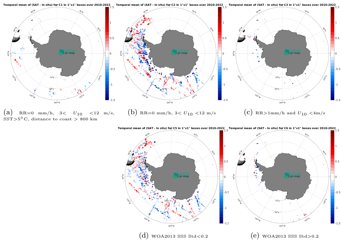
Figure 14: Temporal mean gridded over spatial boxes of size 1^\circ \times 1^\circ of \Delta\text{SSS} (SMOS SSS L3 v332 - 9 Days (CATDS-CPDC) - TSG (SAMOS)) for 5 different subdatasets corresponding to:RR=0 mm/h, 3 < U_{10} < 12 m/s, SST > 5^\circ\text{C} , distance to coast > 800 km (a), RR=0 mm/h, 3 < U_{10} < 12 m/s (b), RR > 1 mm/h and U_{10} < 4 m/s (c), WOA2013 SSS Std < 0.2 (d), WOA2013 SSS Std > 0.2 (e).
