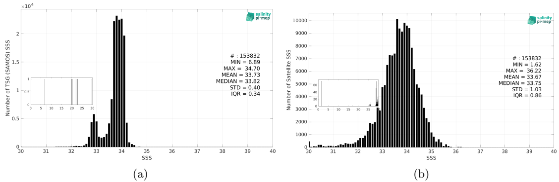
Figure 3: Histograms of SSS from TSG (SAMOS) (a) and SMOS SSS L3 v332 - 9 Days (CATDS-CPDC) (b) considering all match-up pairs per bins of 0.1 over the Southern Ocean Pi-MEP region and for the full satellite product period.
