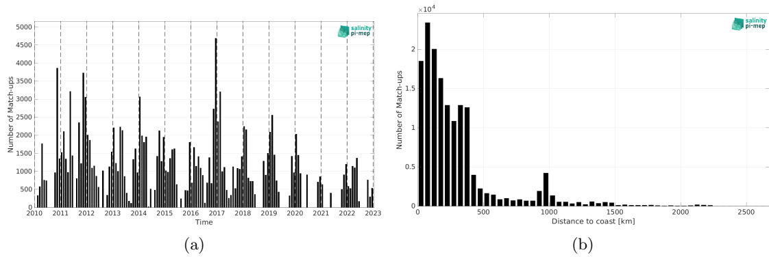
Figure 2: Number of match-ups between TSG (SAMOS) and SMOS SSS L3 v332 - 9 Days (CATDS-CPDC) SSS as a function of time (a) and as function of the distance to coast (b) over the Southern Ocean Pi-MEP region and for the full satellite product period.
