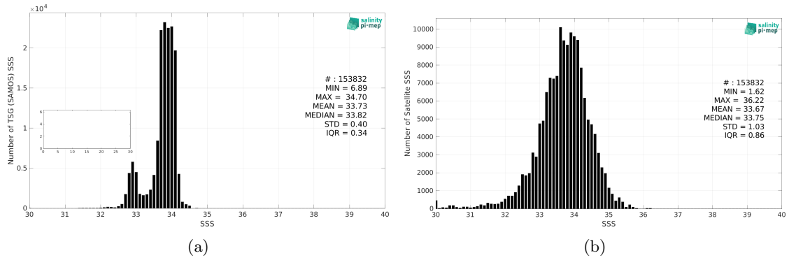
Figure 2: Histograms of SSS from TSG (SAMOS) (a) and SMOS SSS L3 v332 - 9 Days (CATDS-CPDC) (b) considering all match-up pairs per bins of 0.1 over the Southern Ocean Pi-MEP region and for the full satellite product period.
