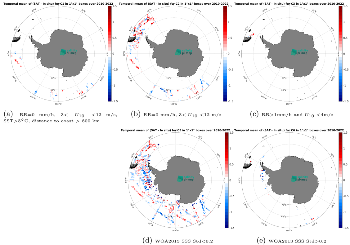
Figure 12: Temporal mean gridded over spatial boxes of size 1^{\circ}\times 1^{\circ} of \Delta\text{SSS} (SMOS SSS L3 v332 - 9 Days (CATDS-CPDC) - TSG (SAMOS)) for 5 different subdatasets corresponding to:RR=0 mm/h, 3 < U_{10} < 12 m/s, SST >5^{\circ}\text{C} , distance to coast > 800 km (a), RR=0 mm/h, 3 < U_{10} < 12 m/s (b), RR >1 mm/h and U_{10} < 4 m/s (c), WOA2013 SSS Std <0.2 (d), WOA2013 SSS Std >0.2 (e).
