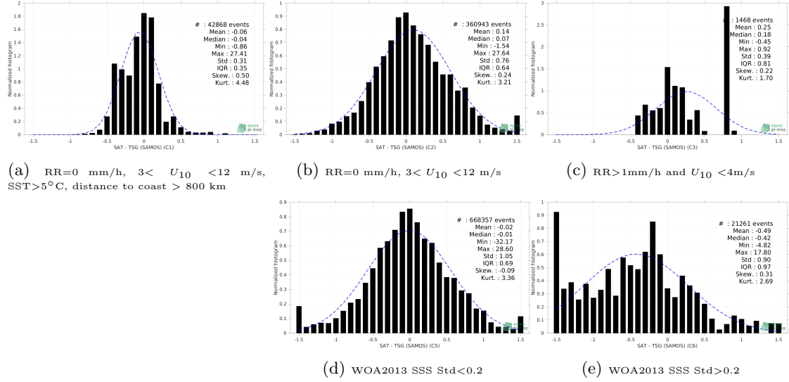
Figure 13: Normalized histogram of \Delta SSS (SMOS SSS L3 v332 - 9 Days (CATDS-CPDC) - TSG (SAMOS)) for 5 different subdatasets corresponding to: RR=0 mm/h, 3 < U_{10} < 12 m/s, SST>5°C, distance to coast > 800 km (a), RR=0 mm/h, 3 < U_{10} < 12 m/s (b), RR>1mm/h and U_{10} < 4 m/s (c), WOA2013 SSS Std<0.2 (d), WOA2013 SSS Std>0.2 (e).
