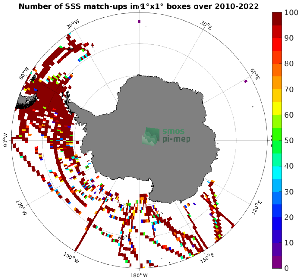
Figure 4: Number of SSS match-ups between TSG (SAMOS) SSS and the SMOS SSS L3 v332 - 9 Days (CATDS-CPDC) SSS product for the Southern Ocean Pi-MEP region over 1^\circ \times 1^\circ boxes and for the full satellite product period.
