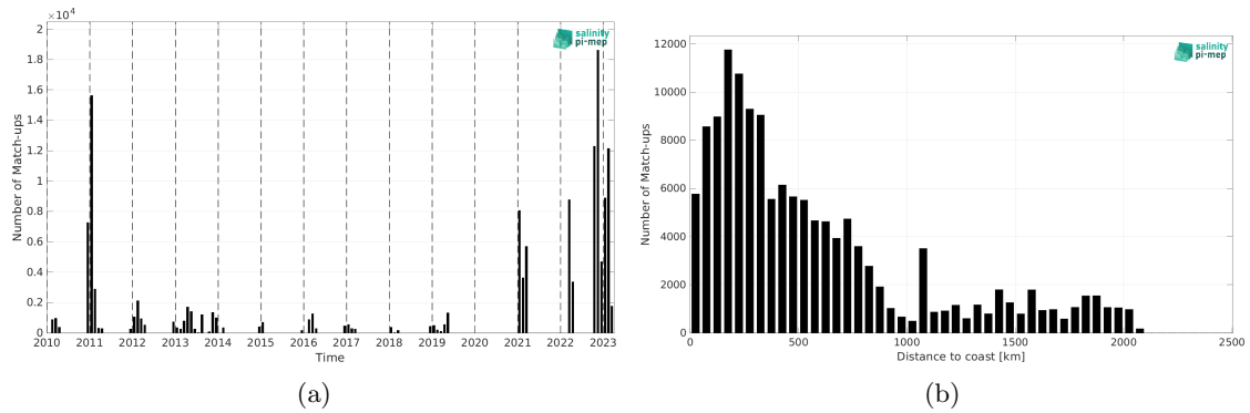
Figure 2: Number of match-ups between TSG (Polarstern) and SMOS SSS L3 v332 - 9 Days (CATDS-CPDC) SSS as a function of time (a) and as function of the distance to coast (b) over the Southern Ocean Pi-MEP region and for the full satellite product period.
