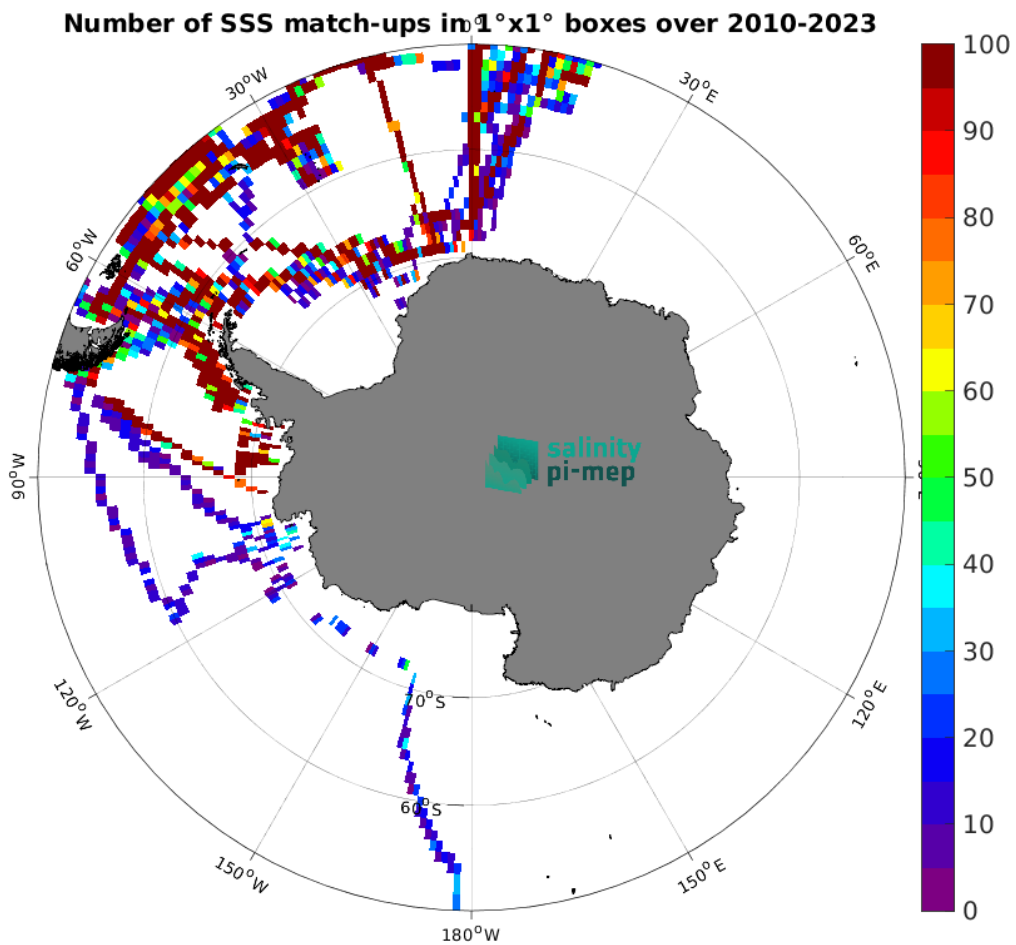
Figure 5: Number of SSS match-ups between TSG (Polarstern) SSS and the SMOS SSS L3 v332 - 9 Days (CATDS-CPDC) SSS product for the Southern Ocean Pi-MEP region over 1^\circ \times 1^\circ boxes and for the full satellite product period.
