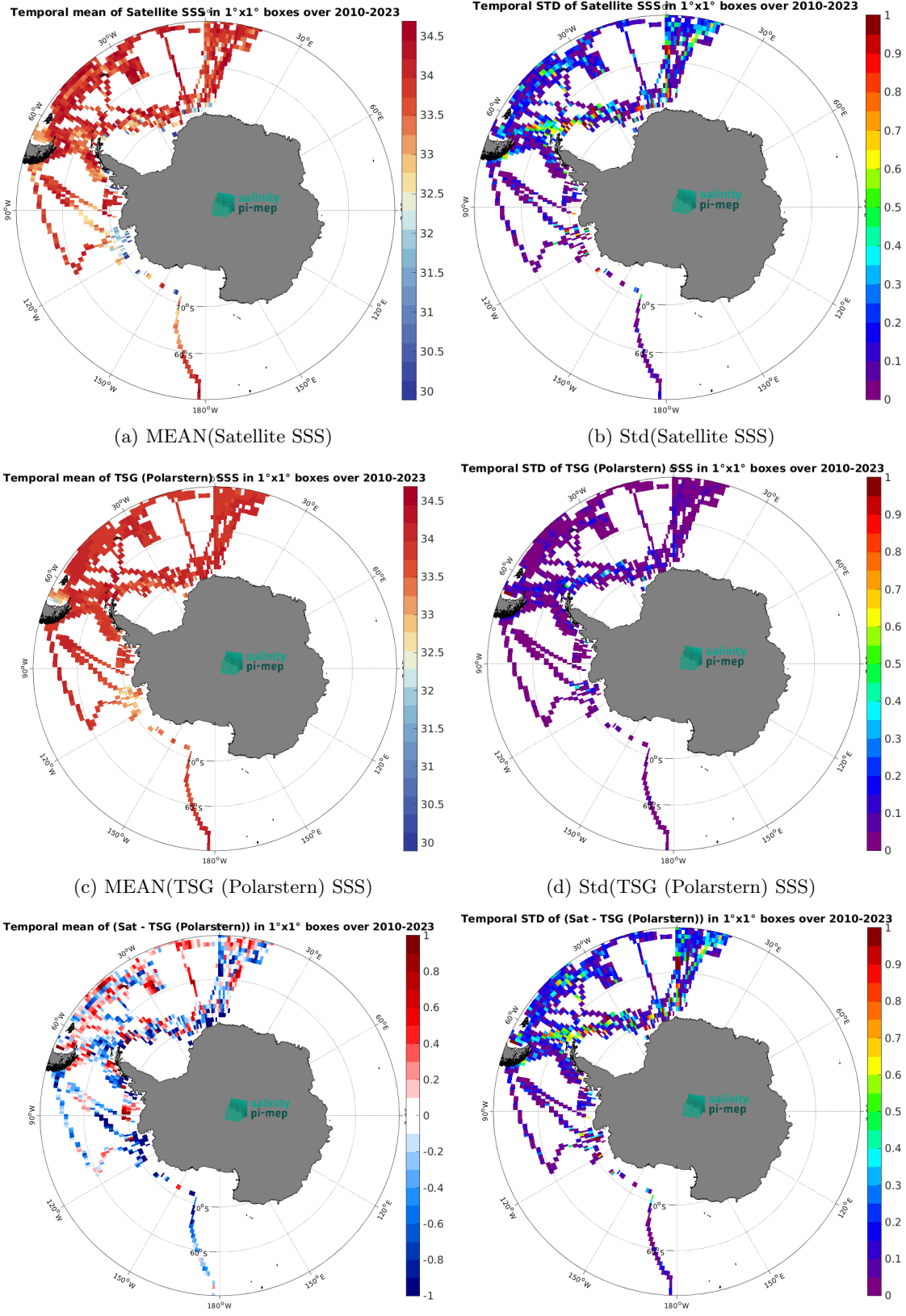
Figure 7: Temporal mean (left) and Std (right) of SSS from SMOS SSS L3 v332 - 9 Days (CATDS-CPDC) (top), TSG (Polarstern) (middle), and of \Delta SSS (Satellite - TSG (Polarstern)). Only match-up pairs are used to generate these maps.
