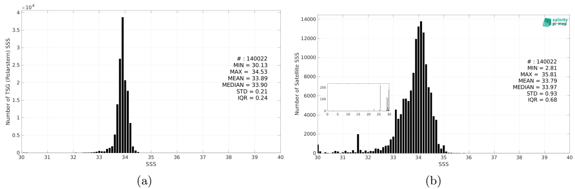
Figure 3: Histograms of SSS from TSG (Polarstern) (a) and SMOS SSS L3 v332 - 9 Days (CATDS-CPDC) (b) considering all match-up pairs per bins of 0.1 over the Southern Ocean Pi-MEP region and for the full satellite product period.
