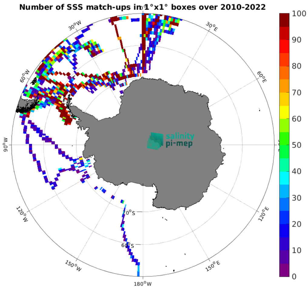
Figure 4: Number of SSS match-ups between TSG (Polarstern) SSS and the SMOS SSS L3 v332 - 9 Days (CATDS-CPDC) SSS product for the Southern Ocean Pi-MEP region over 1^\circ \times 1^\circ boxes and for the full satellite product period.
