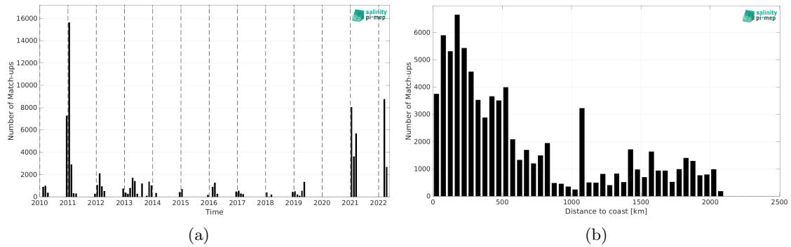
Figure 1: Number of match-ups between TSG (Polarstern) and SMOS SSS L3 v332 - 9 Days (CATDS-CPDC) SSS as a function of time (a) and as function of the distance to coast (b) over the Southern Ocean Pi-MEP region and for the full satellite product period.
