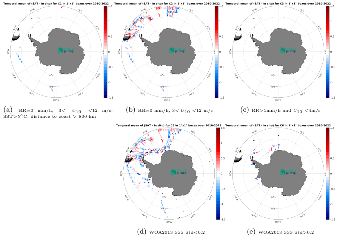
Figure 12: Temporal mean gridded over spatial boxes of size 1^{\circ}\times 1^{\circ} of \Delta\text{SSS} (SMOS SSS L3 v332 - 9 Days (CATDS-CPDC) - TSG (Polarstern)) for 5 different subdatasets corresponding to:RR=0 mm/h, 3 < U_{10} < 12 m/s, SST >5^{\circ}\text{C} , distance to coast > 800 km (a), RR=0 mm/h, 3 < U_{10} < 12 m/s (b), RR >1 mm/h and U_{10} < 4 m/s (c), WOA2013 SSS Std <0.2 (d), WOA2013 SSS Std >0.2 (e).
