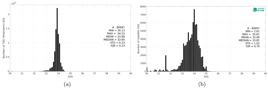
Figure 2: Histograms of SSS from TSG (Polarstern) (a) and SMOS SSS L3 v332 - 9 Days (CATDS-CPDC) (b) considering all match-up pairs per bins of 0.1 over the Southern Ocean Pi-MEP region and for the full satellite product period.
