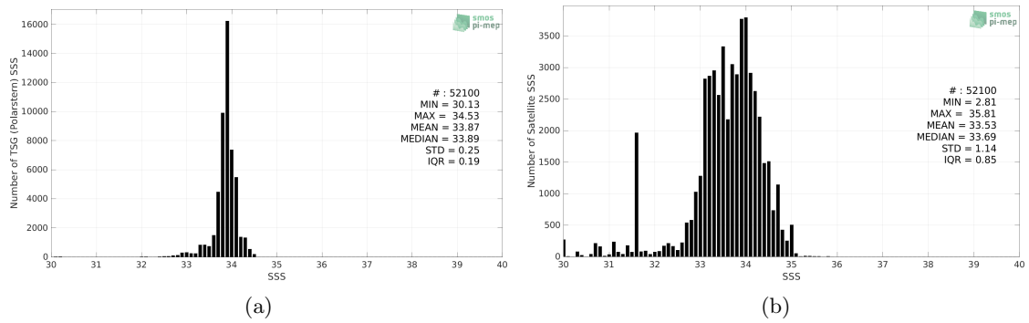
Figure 2: Histograms of SSS from TSG (Polarstern) (a) and SMOS SSS L3 v332 - 9 Days (CATDS-CPDC) (b) considering all match-up pairs per bins of 0.1 over the Southern Ocean Pi-MEP region and for the full satellite product period.
