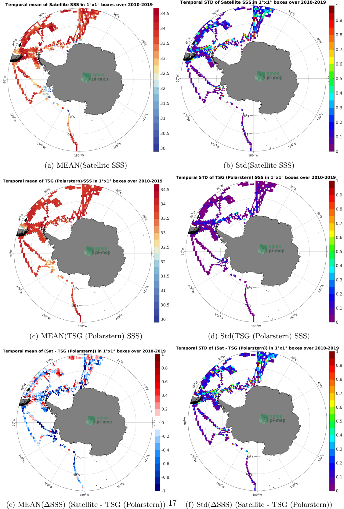
Figure 6: Temporal mean (left) and Std (right) of SSS from SMOS SSS L3 v332 - 9 Days (CATDS-CPDC) (top), TSG (Polarstern) (middle), and of \Delta SSS (Satellite - TSG (Polarstern)). Only match-up pairs are used to generate these maps.
