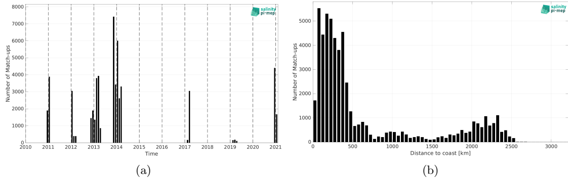
Figure 2: Number of match-ups between TSG (GOSUD-Sailing-ship) and SMOS SSS L3 v332 - 9 Days (CATDS-CPDC) SSS as a function of time (a) and as function of the distance to coast (b) over the Southern Ocean Pi-MEP region and for the full satellite product period.
