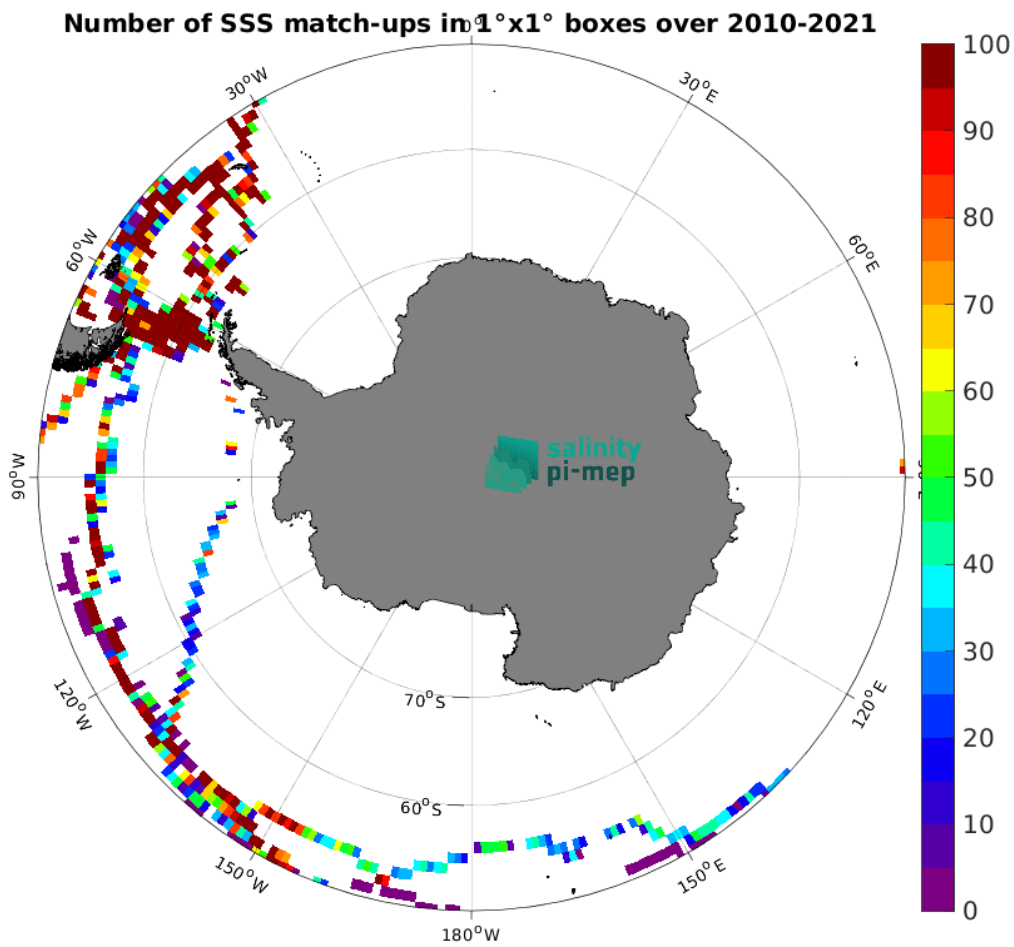
Figure 5: Number of SSS match-ups between TSG (GOSUD-Sailing-ship) SSS and the SMOS SSS L3 v332 - 9 Days (CATDS-CPDC) SSS product for the Southern Ocean Pi-MEP region over 1^\circ \times 1^\circ boxes and for the full satellite product period.
