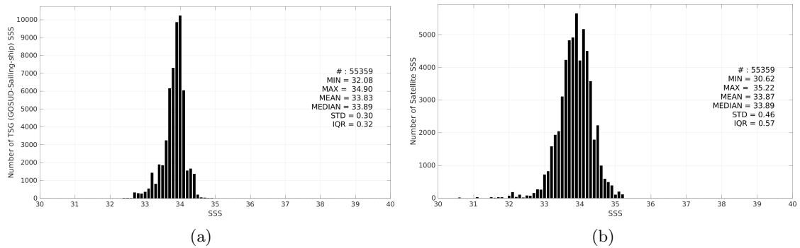
Figure 3: Histograms of SSS from TSG (GOSUD-Sailing-ship) (a) and SMOS SSS L3 v332 - 9 Days (CATDS-CPDC) (b) considering all match-up pairs per bins of 0.1 over the Southern Ocean Pi-MEP region and for the full satellite product period.
