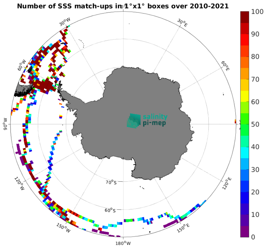
Figure 4: Number of SSS match-ups between TSG (GOSUD-Sailing-ship) SSS and the SMOS SSS L3 v332 - 9 Days (CATDS-CPDC) SSS product for the Southern Ocean Pi-MEP region over 1^\circ \times 1^\circ boxes and for the full satellite product period.
