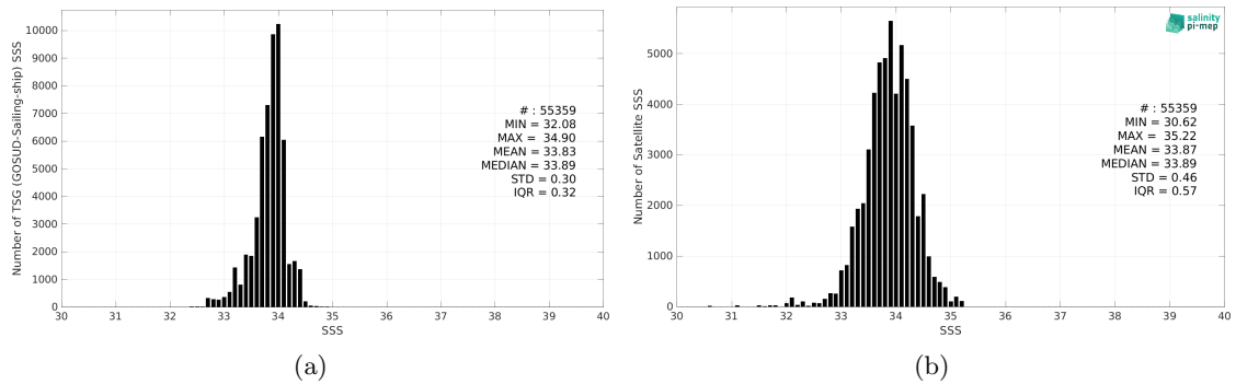
Figure 2: Histograms of SSS from TSG (GOSUD-Sailing-ship) (a) and SMOS SSS L3 v332 - 9 Days (CATDS-CPDC) (b) considering all match-up pairs per bins of 0.1 over the Southern Ocean Pi-MEP region and for the full satellite product period.
