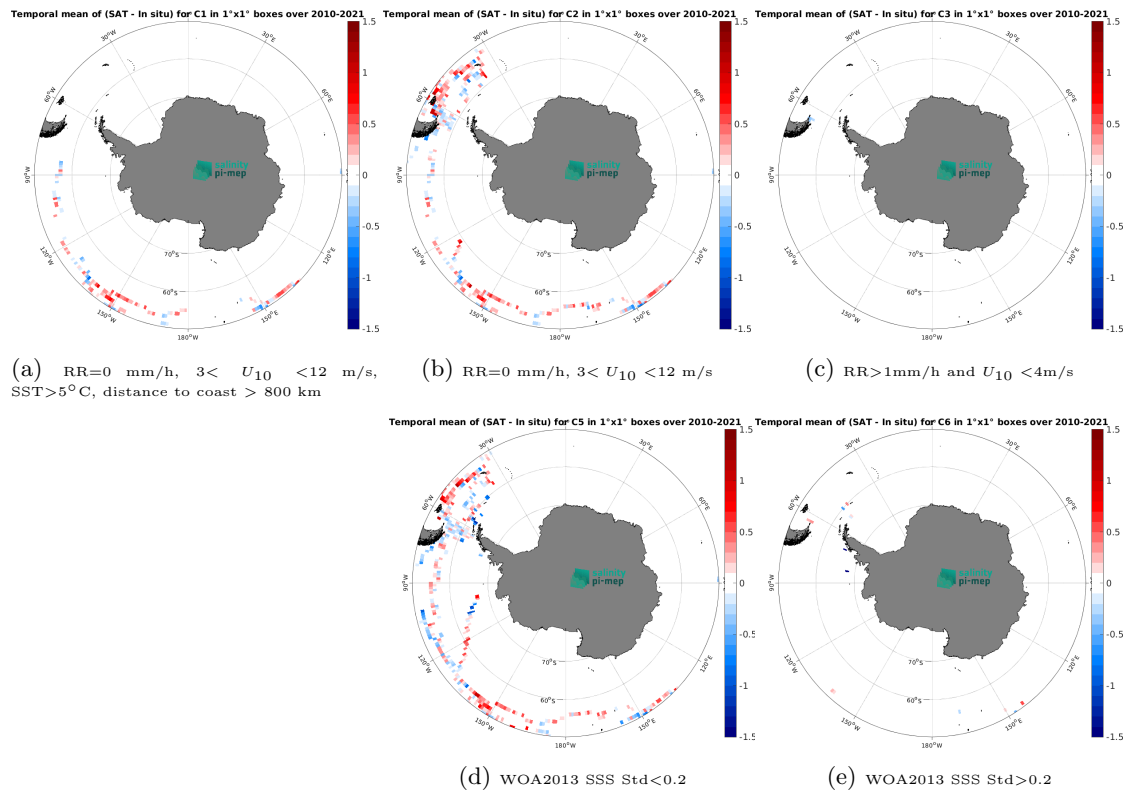
Figure 12: Temporal mean gridded over spatial boxes of size 1^\circ \times 1^\circ of \Delta\text{SSS} (SMOS SSS L3 v332 - 9 Days (CATDS-CPDC) - TSG (GOSUD-Sailing-ship)) for 5 different subdatasets corresponding to: RR=0 mm/h, 3 < U_{10} < 12 m/s, SST > 5^\circ\text{C} , distance to coast > 800 km (a), RR=0 mm/h, 3 < U_{10} < 12 m/s (b), RR > 1 mm/h and U_{10} < 4 m/s (c), WOA2013 SSS Std < 0.2 (d), WOA2013 SSS Std > 0.2 (e).
