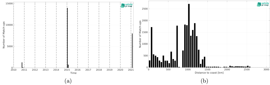
Figure 2: Number of match-ups between TSG (GOSUD-Research-vessel) and SMOS SSS L3 v332 - 9 Days (CATDS-CPDC) SSS as a function of time (a) and as function of the distance to coast (b) over the Southern Ocean Pi-MEP region and for the full satellite product period.
