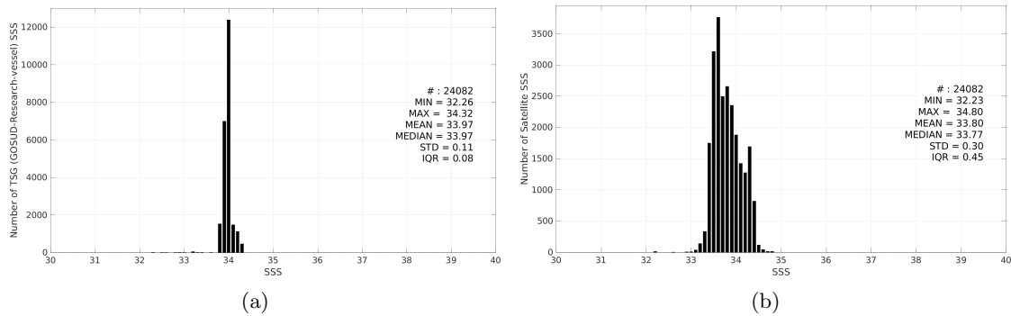
Figure 3: Histograms of SSS from TSG (GOSUD-Research-vessel) (a) and SMOS SSS L3 v332 - 9 Days (CATDS-CPDC) (b) considering all match-up pairs per bins of 0.1 over the Southern Ocean Pi-MEP region and for the full satellite product period.
