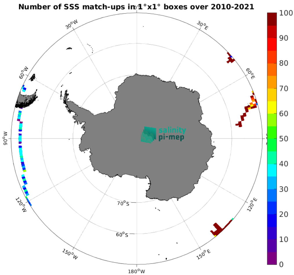
Figure 5: Number of SSS match-ups between TSG (GOSUD-Research-vessel) SSS and the SMOS SSS L3 v332 - 9 Days (CATDS-CPDC) SSS product for the Southern Ocean Pi-MEP region over 1^\circ \times 1^\circ boxes and for the full satellite product period.
