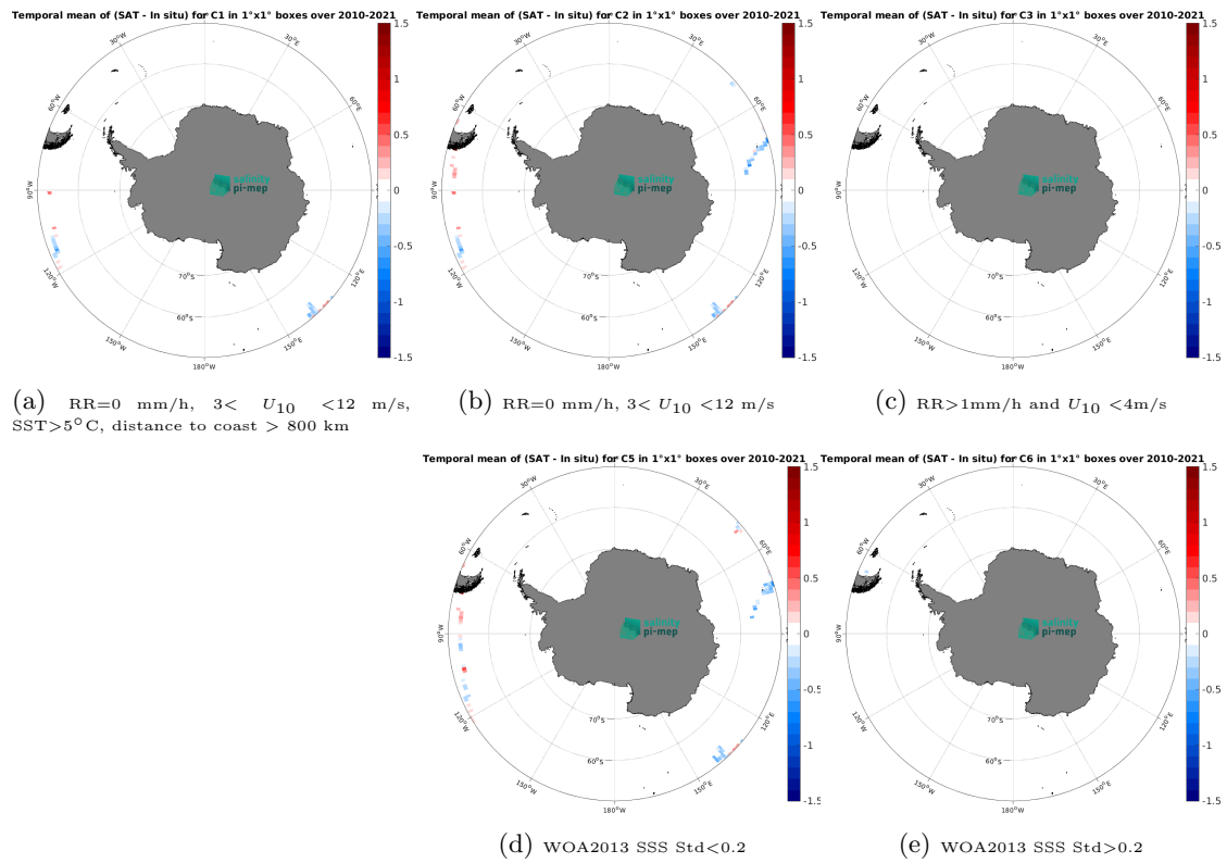
Figure 12: Temporal mean gridded over spatial boxes of size 1^\circ \times 1^\circ of \Delta\text{SSS} (SMOS SSS L3 v332 - 9 Days (CATDS-CPDC) - TSG (GOSUD-Research-vessel)) for 5 different subdatasets corresponding to: RR=0 mm/h, 3 < U_{10} < 12 m/s, SST > 5^\circ\text{C} , distance to coast > 800 km (a), RR=0 mm/h, 3 < U_{10} < 12 m/s (b), RR > 1 mm/h and U_{10} < 4 m/s (c), WOA2013 SSS Std < 0.2 (d), WOA2013 SSS Std > 0.2 (e).
