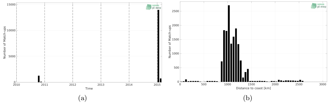
Figure 1: Number of match-ups between TSG (GOSUD-Research-vessel) and SMOS SSS L3 v332 - 9 Days (CATDS-CPDC) SSS as a function of time (a) and as function of the distance to coast (b) over the Southern Ocean Pi-MEP region and for the full satellite product period.
