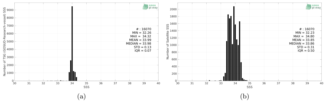
Figure 2: Histograms of SSS from TSG (GOSUD-Research-vessel) (a) and SMOS SSS L3 v332 - 9 Days (CATDS-CPDC) (b) considering all match-up pairs per bins of 0.1 over the Southern Ocean Pi-MEP region and for the full satellite product period.
