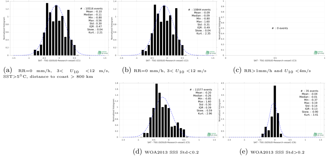
Figure 13: Normalized histogram of \Delta SSS (SMOS SSS L3 v332 - 9 Days (CATDS-CPDC) - TSG (GOSUD-Research-vessel)) for 5 different subdatasets corresponding to: RR=0 mm/h, 3 < U_{10} < 12 m/s, SST > 5°C, distance to coast > 800 km (a), RR=0 mm/h, 3 < U_{10} < 12 m/s (b), RR > 1mm/h and U_{10} < 4 m/s (c), WOA2013 SSS Std < 0.2 (d), WOA2013 SSS Std > 0.2 (e).
