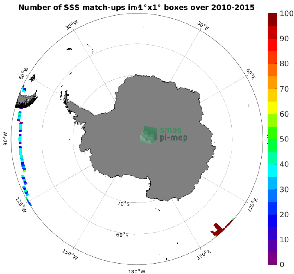
Figure 4: Number of SSS match-ups between TSG (GOSUD-Research-vessel) SSS and the SMOS SSS L3 v332 - 9 Days (CATDS-CPDC) SSS product for the Southern Ocean Pi-MEP region over 1^\circ \times 1^\circ boxes and for the full satellite product period.
