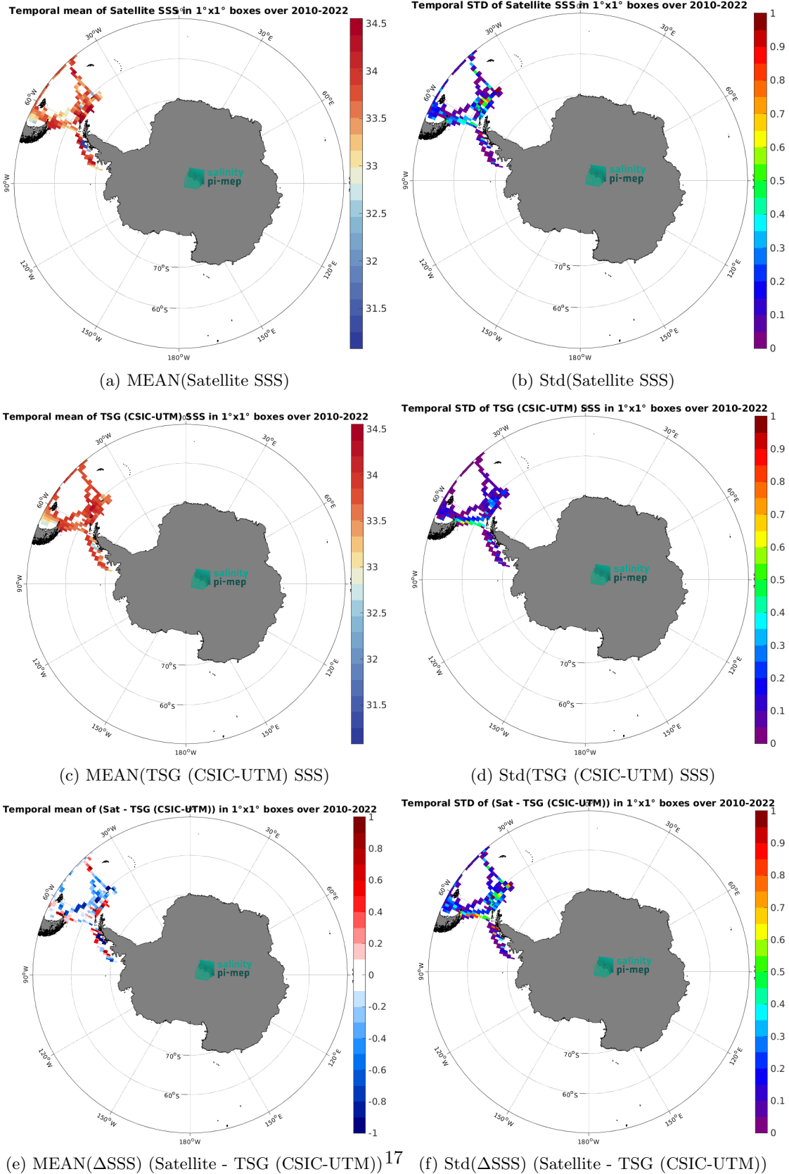
Figure 7: Temporal mean (left) and Std (right) of SSS from SMOS SSS L3 v332 - 9 Days (CATDS-CPDC) (top), TSG (CSIC-UTM) (middle), and of \Delta SSS (Satellite - TSG (CSIC-UTM)). Only match-up pairs are used to generate these maps.
