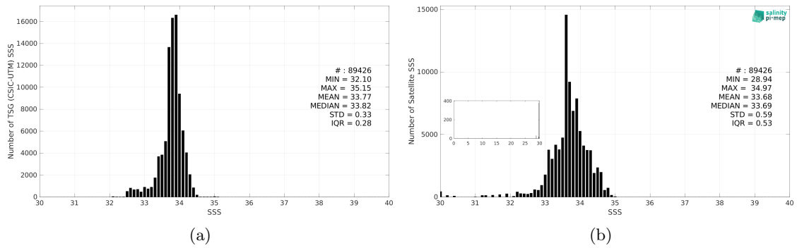
Figure 3: Histograms of SSS from TSG (CSIC-UTM) (a) and SMOS SSS L3 v332 - 9 Days (CATDS-CPDC) (b) considering all match-up pairs per bins of 0.1 over the Southern Ocean Pi-MEP region and for the full satellite product period.
