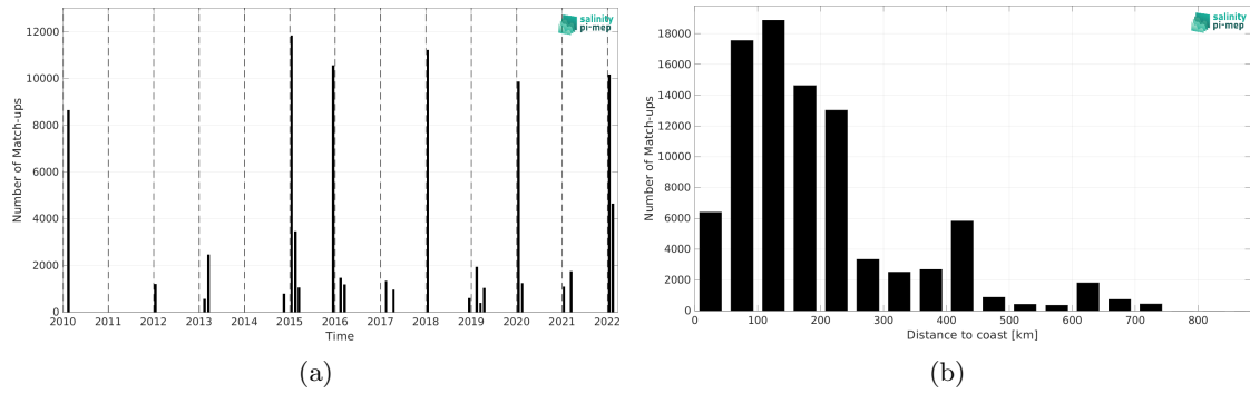
Figure 2: Number of match-ups between TSG (CSIC-UTM) and SMOS SSS L3 v332 - 9 Days (CATDS-CPDC) SSS as a function of time (a) and as function of the distance to coast (b) over the Southern Ocean Pi-MEP region and for the full satellite product period.
