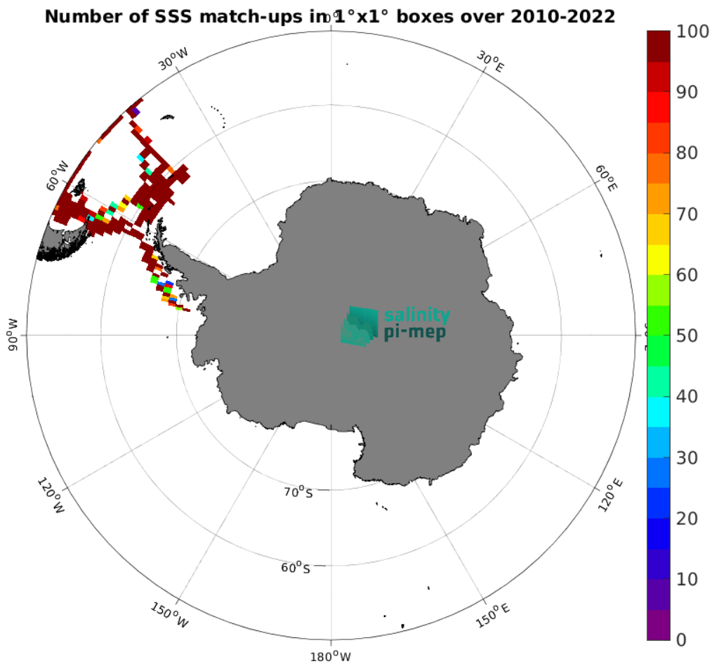
Figure 5: Number of SSS match-ups between TSG (CSIC-UTM) SSS and the SMOS SSS L3 v332 - 9 Days (CATDS-CPDC) SSS product for the Southern Ocean Pi-MEP region over 1^\circ \times 1^\circ boxes and for the full satellite product period.
