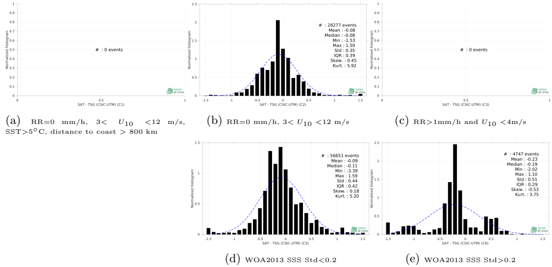
Figure 13: Normalized histogram of \Delta SSS (SMOS SSS L3 v332 - 9 Days (CATDS-CPDC) - TSG (CSIC-UTM)) for 5 different subdatasets corresponding to: RR=0 mm/h, 3 < U_{10} < 12 m/s, SST > 5°C, distance to coast > 800 km (a), RR=0 mm/h, 3 < U_{10} < 12 m/s (b), RR > 1mm/h and U_{10} < 4 m/s (c), WOA2013 SSS Std < 0.2 (d), WOA2013 SSS Std > 0.2 (e).
