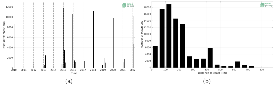
Figure 1: Number of match-ups between TSG (CSIC-UTM) and SMOS SSS L3 v332 - 9 Days (CATDS-CPDC) SSS as a function of time (a) and as function of the distance to coast (b) over the Southern Ocean Pi-MEP region and for the full satellite product period.
