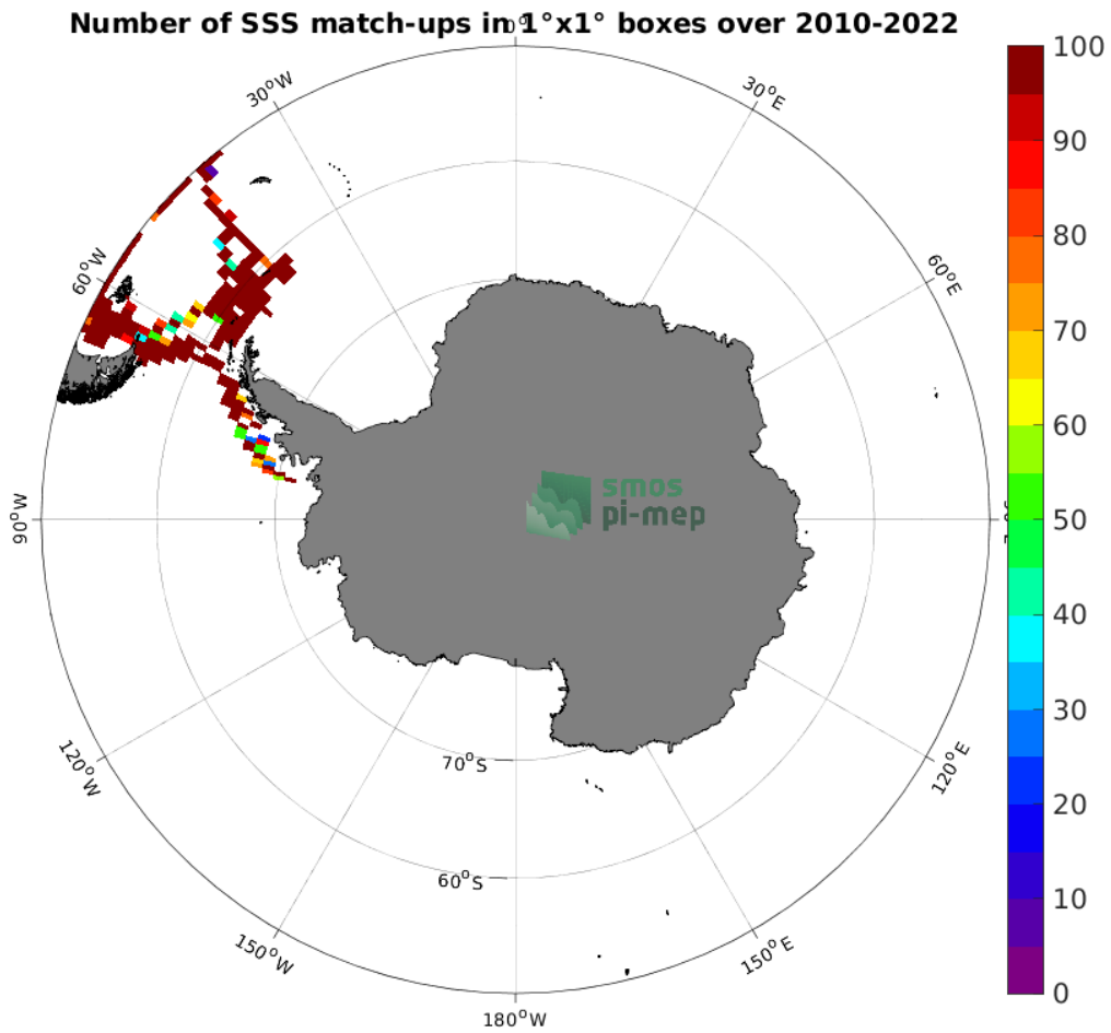
Figure 4: Number of SSS match-ups between TSG (CSIC-UTM) SSS and the SMOS SSS L3 v332 - 9 Days (CATDS-CPDC) SSS product for the Southern Ocean Pi-MEP region over 1^\circ \times 1^\circ boxes and for the full satellite product period.
