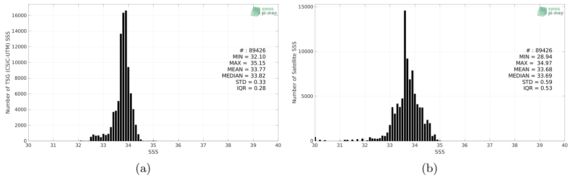
Figure 2: Histograms of SSS from TSG (CSIC-UTM) (a) and SMOS SSS L3 v332 - 9 Days (CATDS-CPDC) (b) considering all match-up pairs per bins of 0.1 over the Southern Ocean Pi-MEP region and for the full satellite product period.
