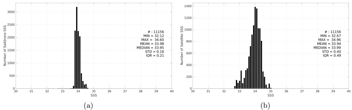
Figure 3: Histograms of SSS from Saildrone (a) and SMOS SSS L3 v332 - 9 Days (CATDS-CPDC) (b) considering all match-up pairs per bins of 0.1 over the Southern Ocean Pi-MEP region and for the full satellite product period.
