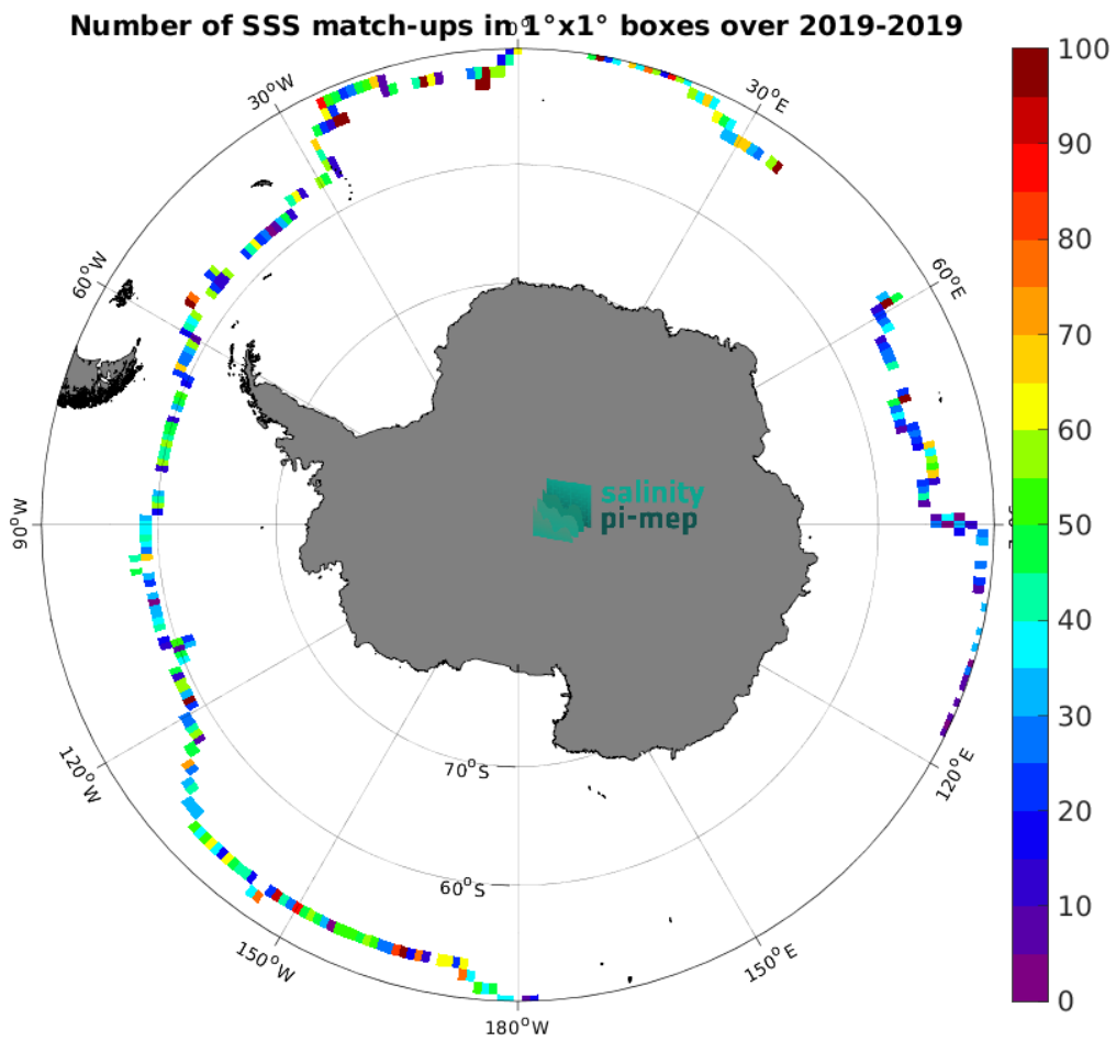
Figure 5: Number of SSS match-ups between Saildrone SSS and the SMOS SSS L3 v332 - 9 Days (CATDS-CPDC) SSS product for the Southern Ocean Pi-MEP region over 1^\circ \times 1^\circ boxes and for the full satellite product period.
