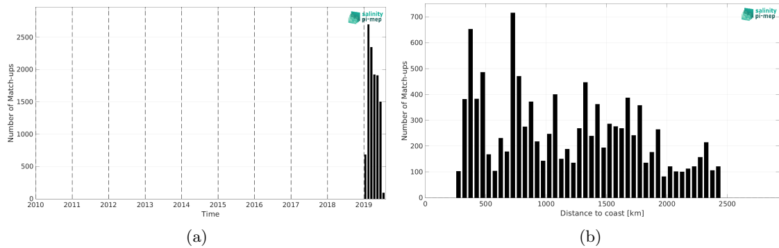
Figure 2: Number of match-ups between Saildrone and SMOS SSS L3 v332 - 9 Days (CATDS-CPDC) SSS as a function of time (a) and as function of the distance to coast (b) over the Southern Ocean Pi-MEP region and for the full satellite product period.
