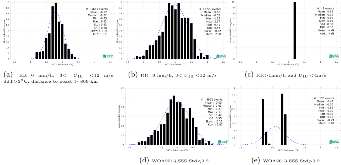
Figure 15: Normalized histogram of \Delta SSS (SMOS SSS L3 v332 - 9 Days (CATDS-CPDC) - Saildrone) for 5 different subdatasets corresponding to: RR=0 mm/h, 3 < U_{10} < 12 m/s, SST > 5°C, distance to coast > 800 km (a), RR=0 mm/h, 3 < U_{10} < 12 m/s (b), RR > 1mm/h and U_{10} < 4 m/s (c), WOA2013 SSS Std < 0.2 (d), WOA2013 SSS Std > 0.2 (e).
