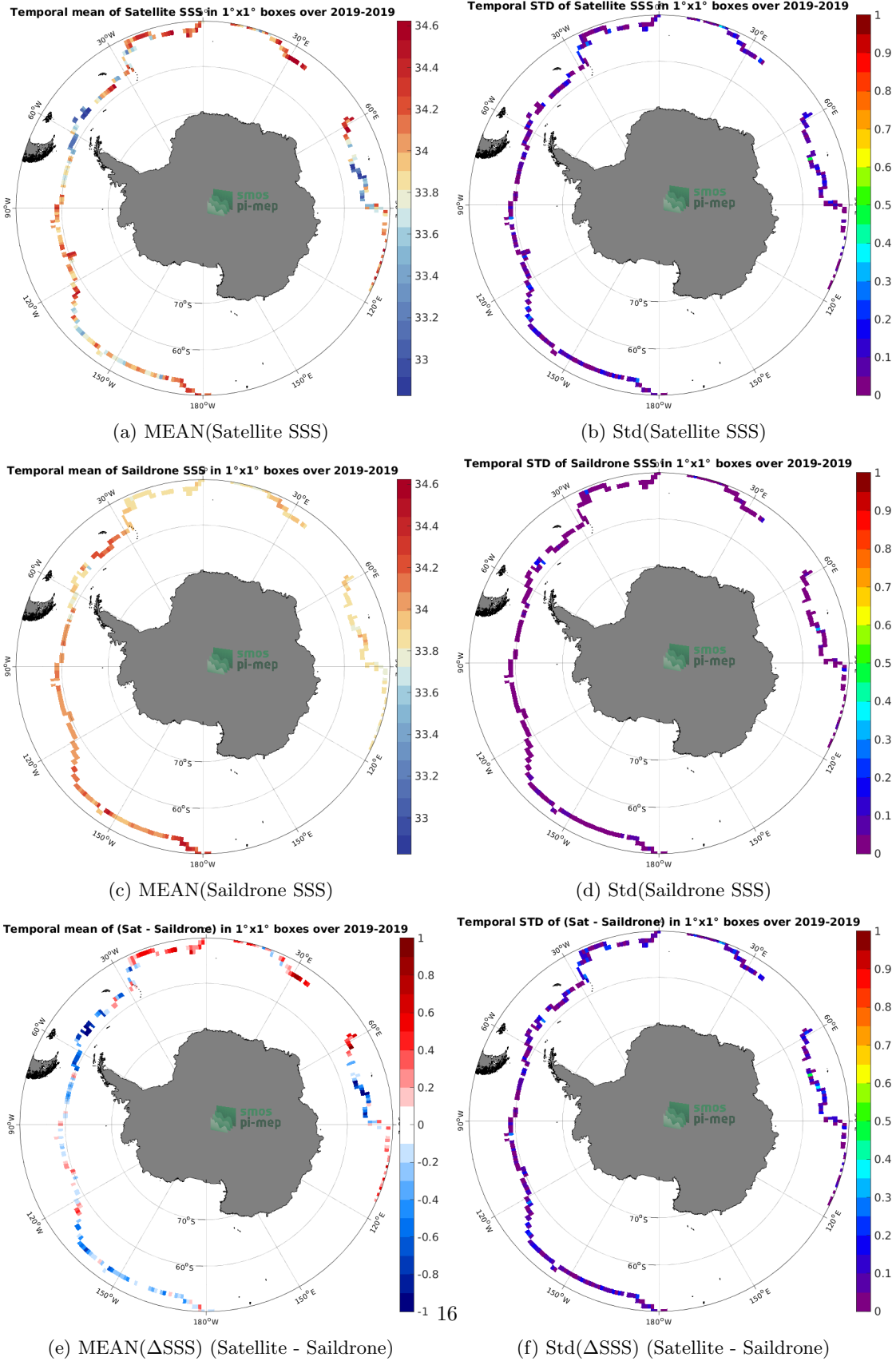
Figure 6: Temporal mean (left) and Std (right) of SSS from SMOS SSS L3 v332 - 9 Days (CATDS-CPDC) (top), Saildrone (middle), and of \Delta SSS (Satellite - Saildrone). Only match-up pairs are used to generate these maps.
