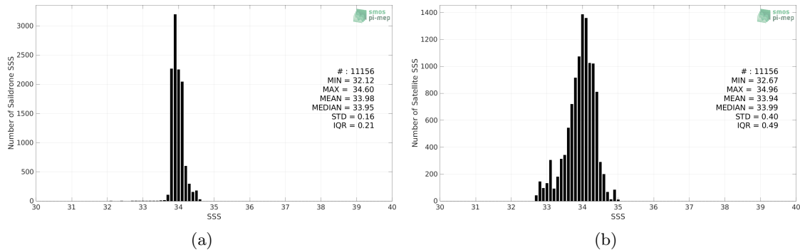
Figure 2: Histograms of SSS from Saildrone (a) and SMOS SSS L3 v332 - 9 Days (CATDS-CPDC) (b) considering all match-up pairs per bins of 0.1 over the Southern Ocean Pi-MEP region and for the full satellite product period.
