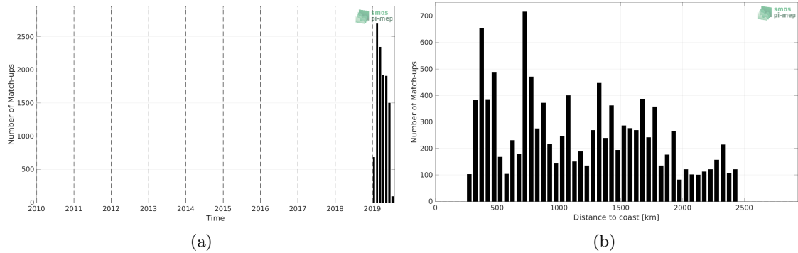
Figure 1: Number of match-ups between Saildrone and SMOS SSS L3 v332 - 9 Days (CATDS-CPDC) SSS as a function of time (a) and as function of the distance to coast (b) over the Southern Ocean Pi-MEP region and for the full satellite product period.
