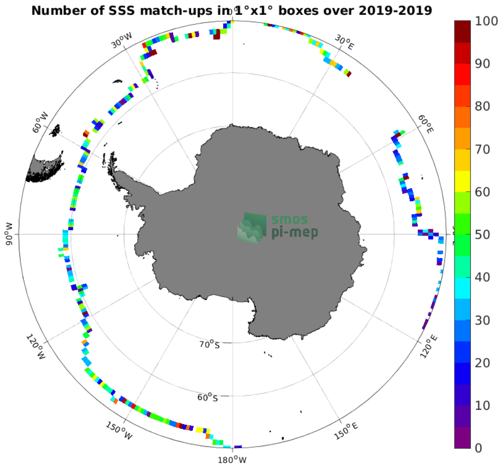
Figure 4: Number of SSS match-ups between Saildrone SSS and the SMOS SSS L3 v332 - 9 Days (CATDS-CPDC) SSS product for the Southern Ocean Pi-MEP region over 1^\circ \times 1^\circ boxes and for the full satellite product period.
