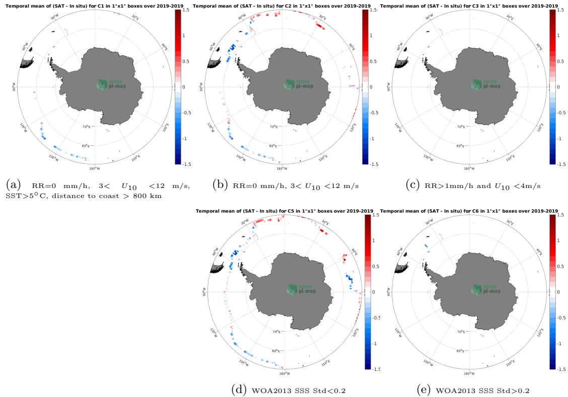
Figure 12: Temporal mean gridded over spatial boxes of size 1^{\circ}\times 1^{\circ} of \Delta\text{SSS} (SMOS SSS L3 v332 - 9 Days (CATDS-CPDC) - Sairdrone) for 5 different subdatasets corresponding to:RR=0 mm/h, 3 < U_{10} < 12 m/s, SST >5^{\circ}\text{C} , distance to coast > 800 km (a), RR=0 mm/h, 3 < U_{10} < 12 m/s (b), RR >1 mm/h and U_{10} < 4 m/s (c), WOA2013 SSS Std <0.2 (d), WOA2013 SSS Std >0.2 (e).
