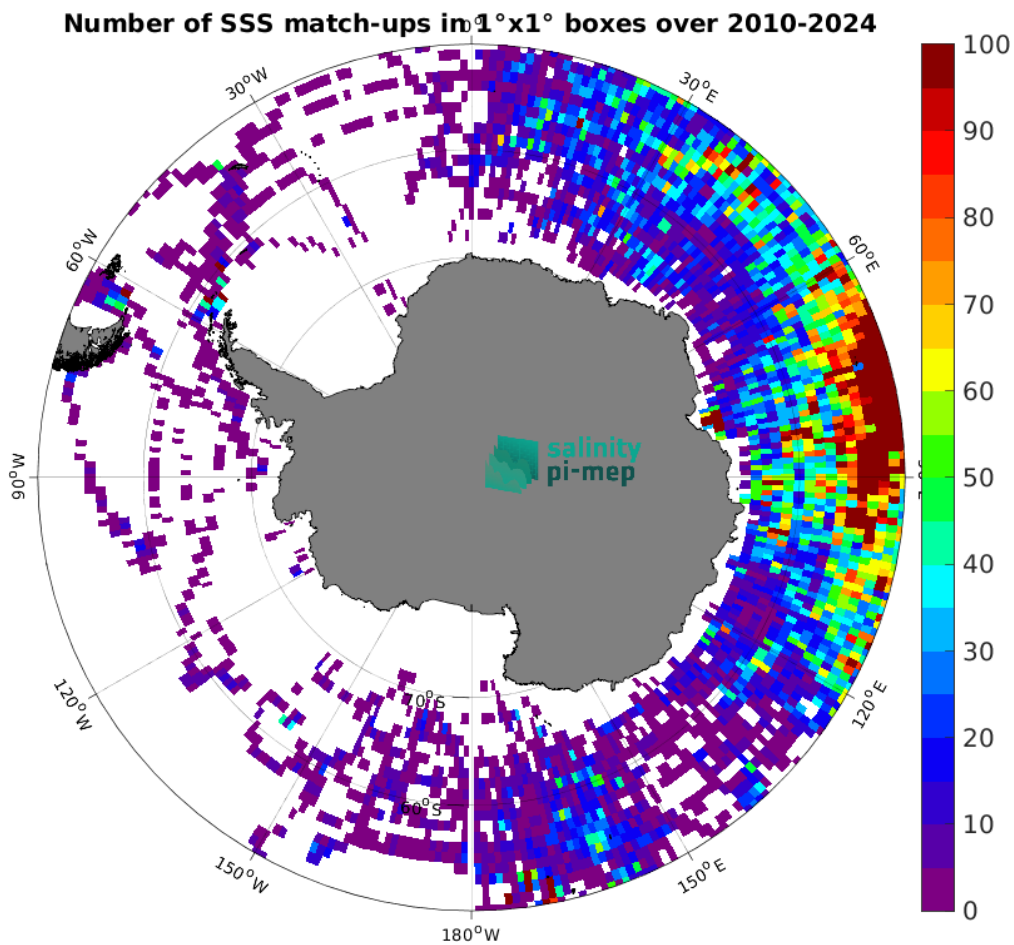
Figure 5: Number of SSS match-ups between Marine mammals SSS and the SMOS SSS L3 v332 - 9 Days (CATDS-CPDC) SSS product for the Southern Ocean Pi-MEP region over 1^{\circ} \times 1^{\circ} boxes and for the full satellite product period.
