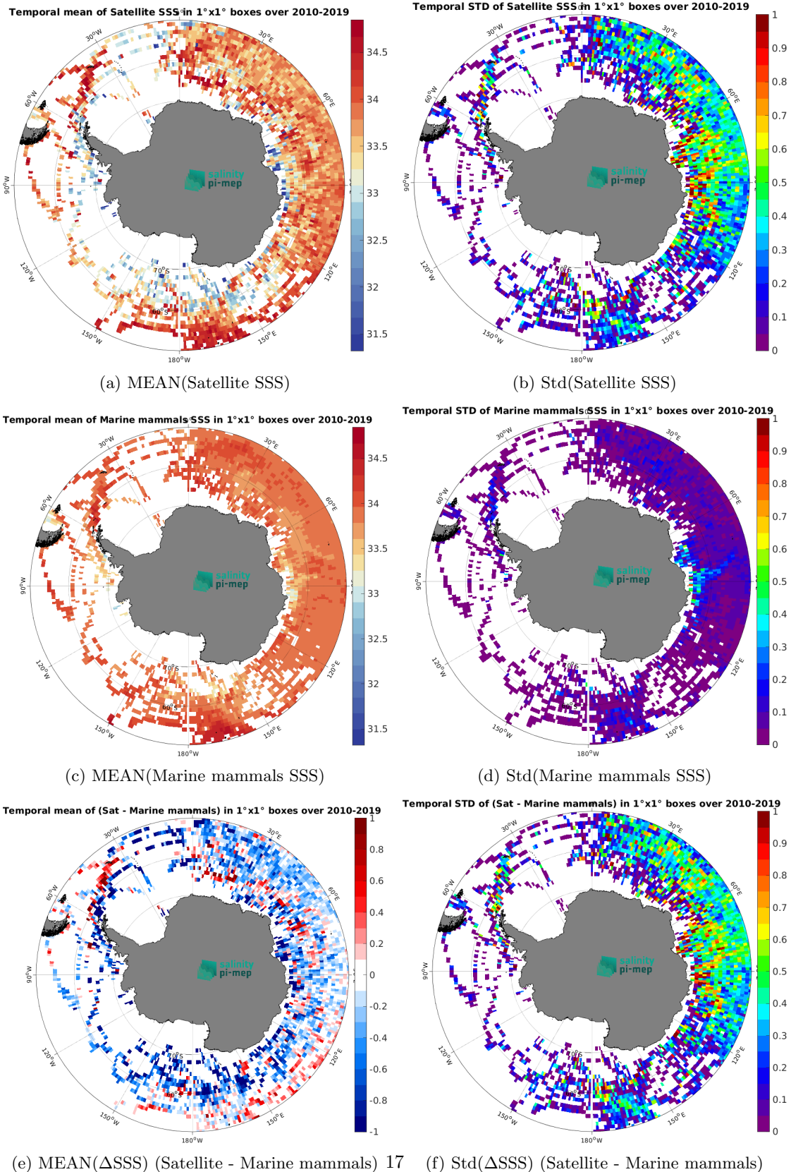
Figure 6: Temporal mean (left) and Std (right) of SSS from SMOS SSS L3 v332 - 9 Days (CATDS-CPDC) (top), Marine mammals (middle), and of \Delta SSS (Satellite - Marine mammals). Only match-up pairs are used to generate these maps.
