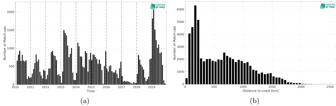
Figure 1: Number of match-ups between Marine mammals and SMOS SSS L3 v332 - 9 Days (CATDS-CPDC) SSS as a function of time (a) and as function of the distance to coast (b) over the Southern Ocean Pi-MEP region and for the full satellite product period.
