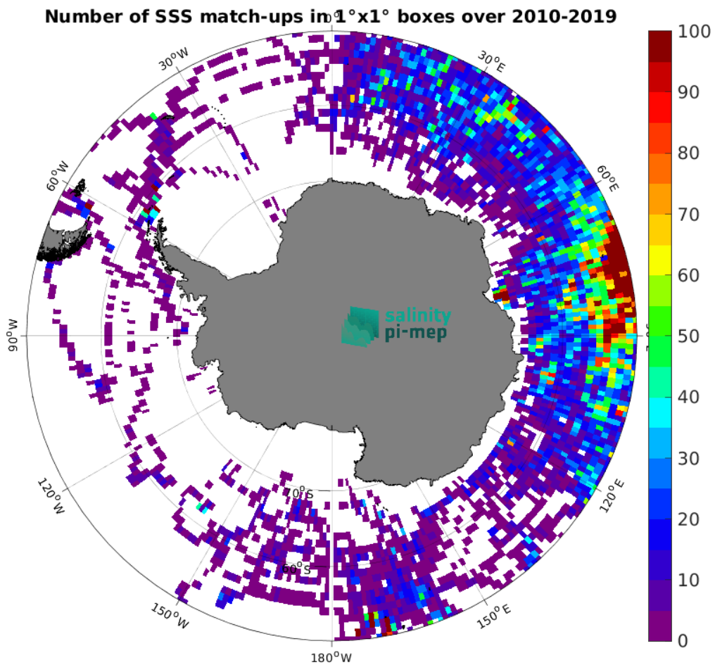
Figure 4: Number of SSS match-ups between Marine mammals SSS and the SMOS SSS L3 v332 - 9 Days (CATDS-CPDC) SSS product for the Southern Ocean Pi-MEP region over 1^\circ \times 1^\circ boxes and for the full satellite product period.
