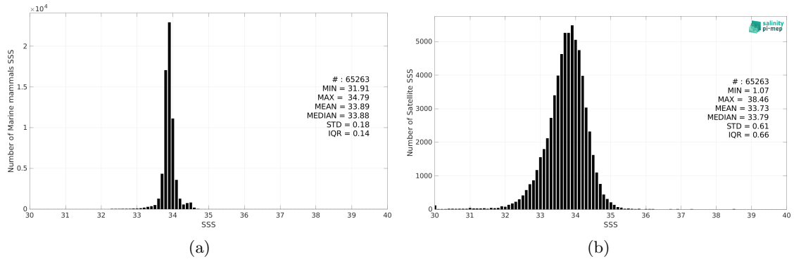
Figure 2: Histograms of SSS from Marine mammals (a) and SMOS SSS L3 v332 - 9 Days (CATDS-CPDC) (b) considering all match-up pairs per bins of 0.1 over the Southern Ocean Pi-MEP region and for the full satellite product period.
