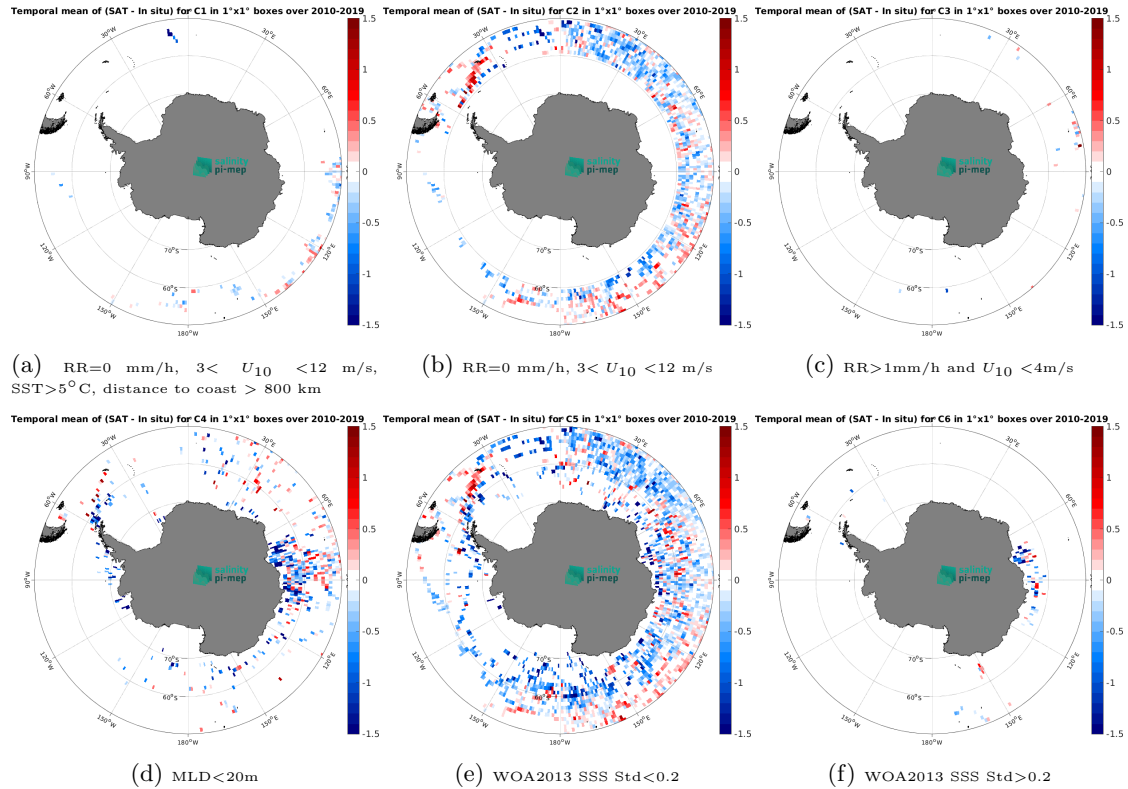
Figure 12: Temporal mean gridded over spatial boxes of size 1^{\circ}\times 1^{\circ} of \Delta\text{SSS} (SMOS SSS L3 v332 - 9 Days (CATDS-CPDC) - Marine mammals) for 6 different subdatasets corresponding to: RR=0 mm/h, 3 < U_{10} < 12 m/s, SST > 5^{\circ}\text{C} , distance to coast > 800 km (a), RR=0 mm/h, 3 < U_{10} < 12 m/s (b), RR > 1\text{mm/h} and U_{10} < 4\text{m/s} (c), MLD < 20\text{m} (d), WOA2013 SSS Std < 0.2 (e), WOA2013 SSS Std > 0.2 (f).
