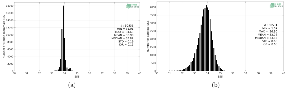
Figure 2: Histograms of SSS from Marine mammals (a) and SMOS SSS L3 v332 - 9 Days (CATDS-CPDC) (b) considering all match-up pairs per bins of 0.1 over the Southern Ocean Pi-MEP region and for the full satellite product period.
