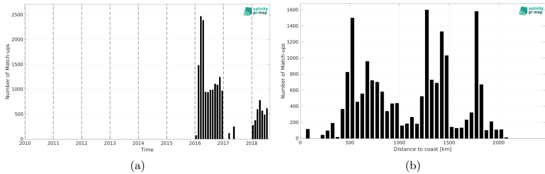
Figure 2: Number of match-ups between Surface drifters and SMOS SSS L3 v332 - 9 Days (CATDS-CPDC) SSS as a function of time (a) and as function of the distance to coast (b) over the Southern Ocean Pi-MEP region and for the full satellite product period.
