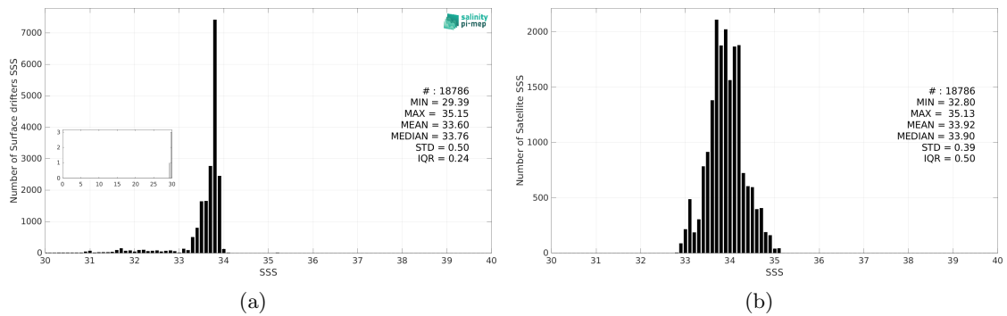
Figure 3: Histograms of SSS from Surface drifters (a) and SMOS SSS L3 v332 - 9 Days (CATDS-CPDC) (b) considering all match-up pairs per bins of 0.1 over the Southern Ocean Pi-MEP region and for the full satellite product period.
