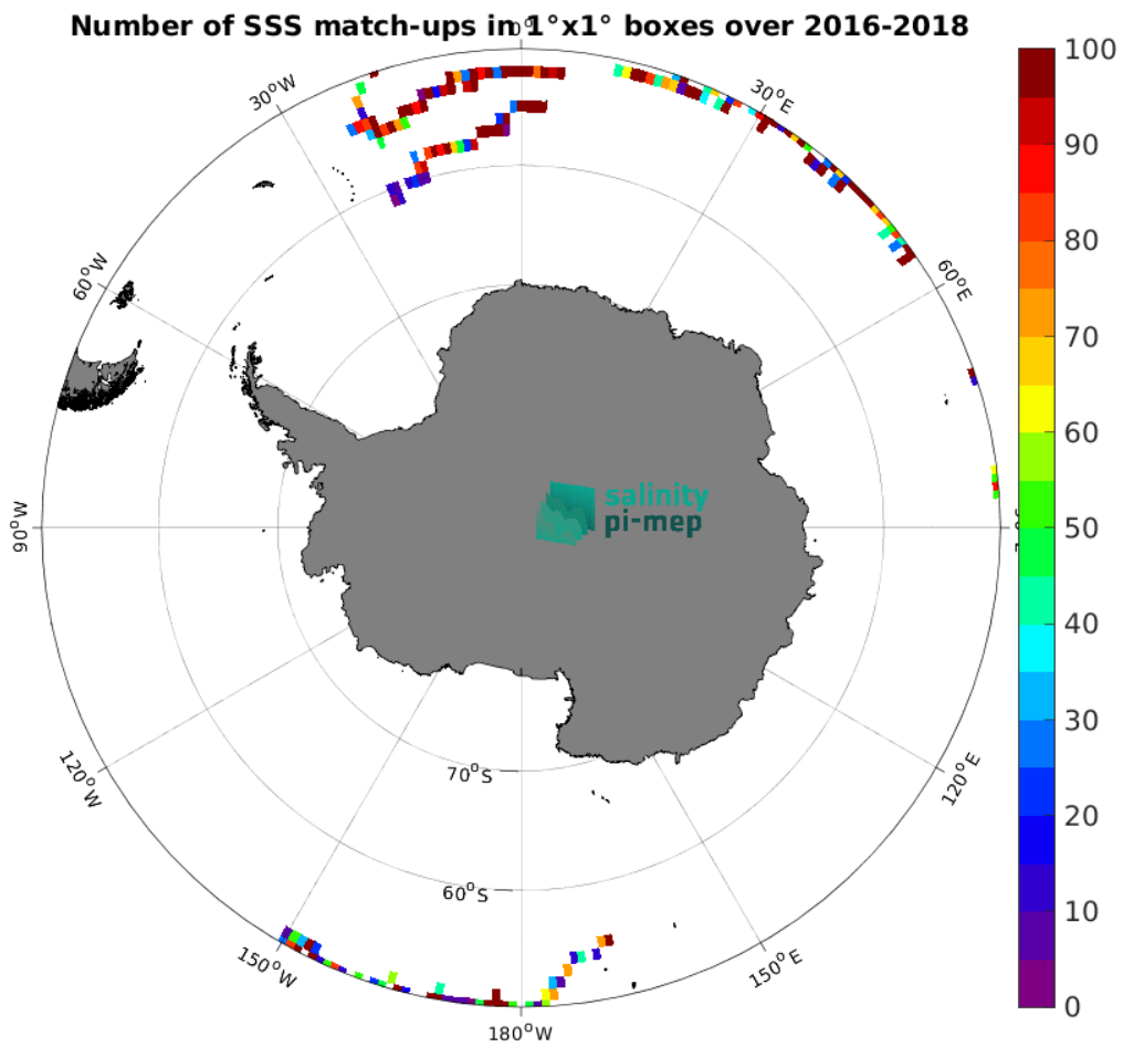
Figure 3: Number of SSS match-ups between Surface drifters SSS and the SMOS SSS L3 v332 - 9 Days (CATDS-CPDC) SSS product for the Southern Ocean Pi-MEP region over 1^\circ \times 1^\circ boxes and for the full satellite product period.
