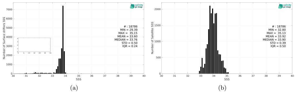
Figure 2: Histograms of SSS from Surface drifters (a) and SMOS SSS L3 v332 - 9 Days (CATDS-CPDC) (b) considering all match-up pairs per bins of 0.1 over the Southern Ocean Pi-MEP region and for the full satellite product period.
