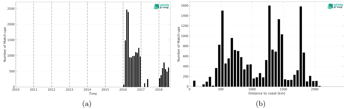
Figure 1: Number of match-ups between Surface drifters and SMOS SSS L3 v332 - 9 Days (CATDS-CPDC) SSS as a function of time (a) and as function of the distance to coast (b) over the Southern Ocean Pi-MEP region and for the full satellite product period.
