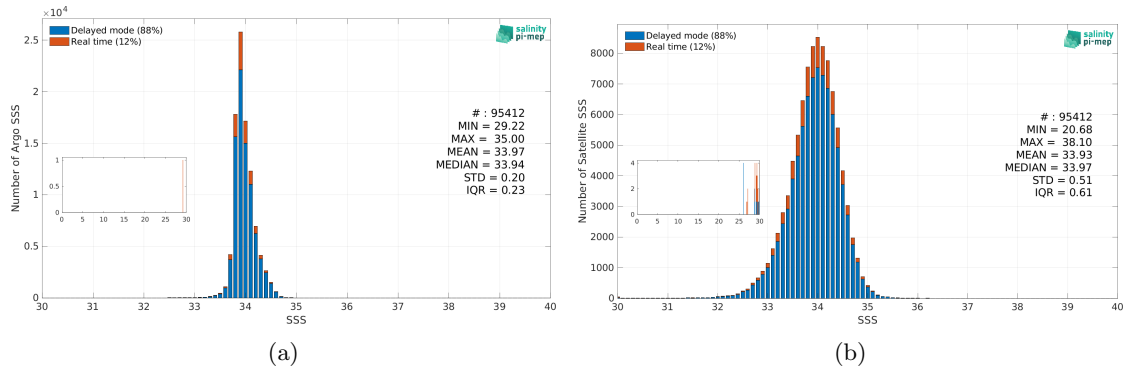
Figure 3: Histograms of SSS from Argo (a) and SMOS SSS L3 v332 - 9 Days (CATDS-CPDC) (b) considering all match-up pairs per bins of 0.1 over the Southern Ocean Pi-MEP region and for the full satellite product period.
