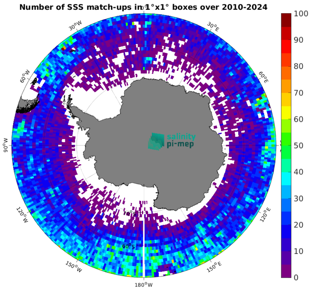
Figure 5: Number of SSS match-ups between Argo SSS and the SMOS SSS L3 v332 - 9 Days (CATDS-CPDC) SSS product for the Southern Ocean Pi-MEP region over 1^\circ \times 1^\circ boxes and for the full satellite product period.
