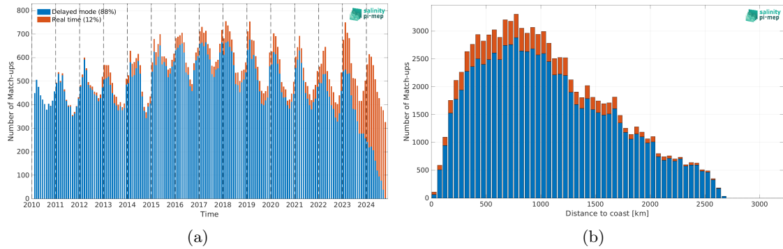
Figure 2: Number of match-ups between Argo and SMOS SSS L3 v332 - 9 Days (CATDS-CPDC) SSS as a function of time (a) and as function of the distance to coast (b) over the Southern Ocean Pi-MEP region and for the full satellite product period.
