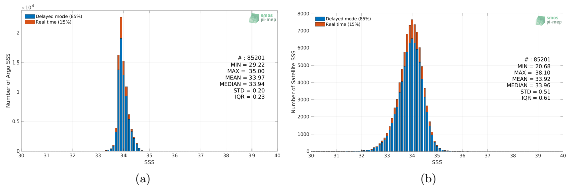
Figure 2: Histograms of SSS from Argo (a) and SMOS SSS L3 v332 - 9 Days (CATDS-CPDC) (b) considering all match-up pairs per bins of 0.1 over the Southern Ocean Pi-MEP region and for the full satellite product period.
