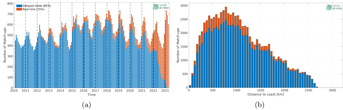
Figure 1: Number of match-ups between Argo and SMOS SSS L3 v332 - 9 Days (CATDS-CPDC) SSS as a function of time (a) and as function of the distance to coast (b) over the Southern Ocean Pi-MEP region and for the full satellite product period.
