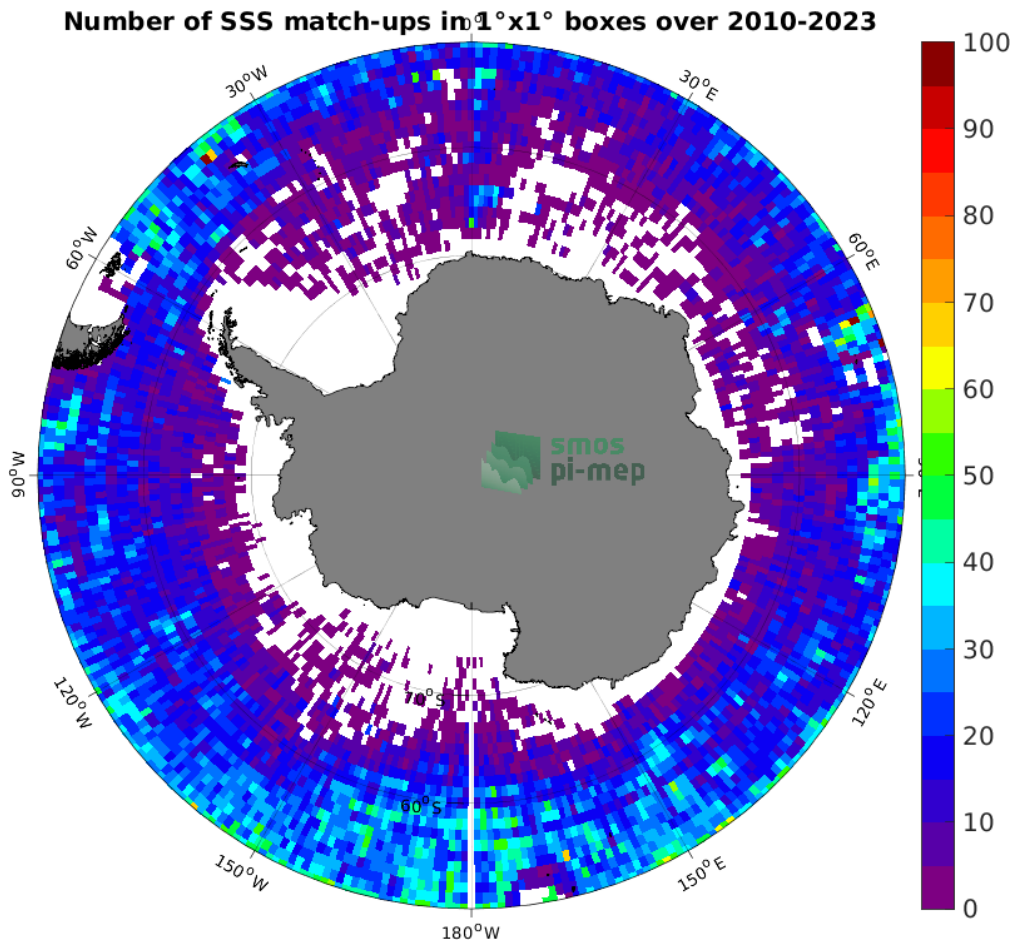
Figure 4: Number of SSS match-ups between Argo SSS and the SMOS SSS L3 v332 - 9 Days (CATDS-CPDC) SSS product for the Southern Ocean Pi-MEP region over 1^\circ \times 1^\circ boxes and for the full satellite product period.
