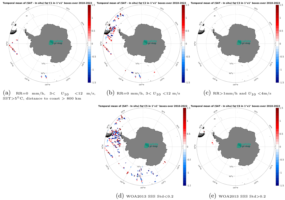
Figure 12: Temporal mean gridded over spatial boxes of size 1^{\circ}\times 1^{\circ} of \Delta\text{SSS} (SMOS SSS L2Q v331 - 0.25 Deg (CATDS-CPDC) - TSG (SAMOS)) for 5 different subdatasets corresponding to:RR=0 mm/h, 3 < U_{10} < 12 m/s, SST >5^{\circ}\text{C} , distance to coast > 800 km (a), RR=0 mm/h, 3 < U_{10} < 12 m/s (b), RR >1 mm/h and U_{10} < 4 m/s (c), WOA2013 SSS Std <0.2 (d), WOA2013 SSS Std >0.2 (e).
