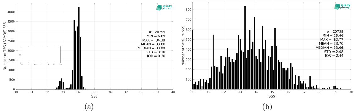
Figure 2: Histograms of SSS from TSG (SAMOS) (a) and SMOS SSS L2Q v331 - 0.25 Deg (CATDS-CPDC) (b) considering all match-up pairs per bins of 0.1 over the Southern Ocean Pi-MEP region and for the full satellite product period.
