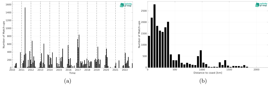
Figure 1: Number of match-ups between TSG (SAMOS) and SMOS SSS L2Q v331 - 0.25 Deg (CATDS-CPDC) SSS as a function of time (a) and as function of the distance to coast (b) over the Southern Ocean Pi-MEP region and for the full satellite product period.
