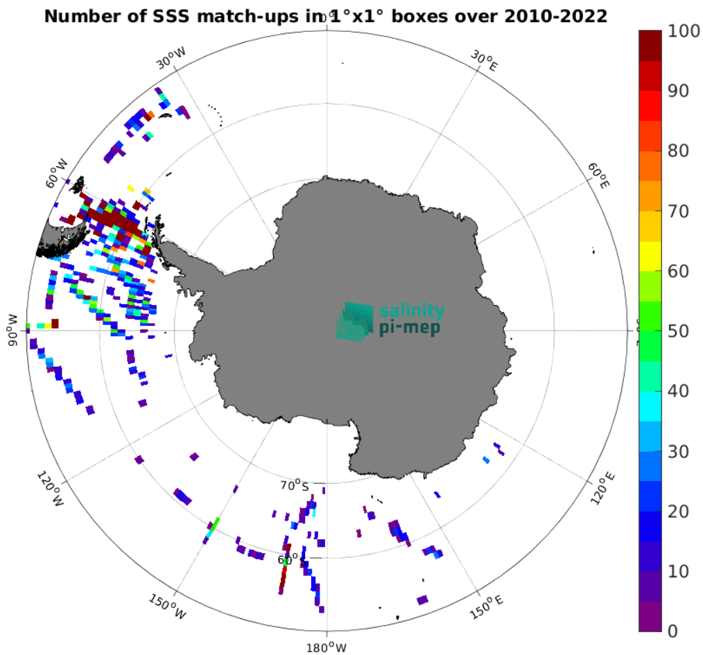
Figure 4: Number of SSS match-ups between TSG (SAMOS) SSS and the SMOS SSS L2Q v331 - 0.25 Deg (CATDS-CPDC) SSS product for the Southern Ocean Pi-MEP region over 1^\circ \times 1^\circ boxes and for the full satellite product period.
