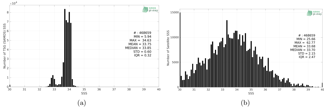
Figure 2: Histograms of SSS from TSG (SAMOS) (a) and SMOS SSS L2Q v331 - 0.25 Deg (CATDS-CPDC) (b) considering all match-up pairs per bins of 0.1 over the Southern Ocean Pi-MEP region and for the full satellite product period.
