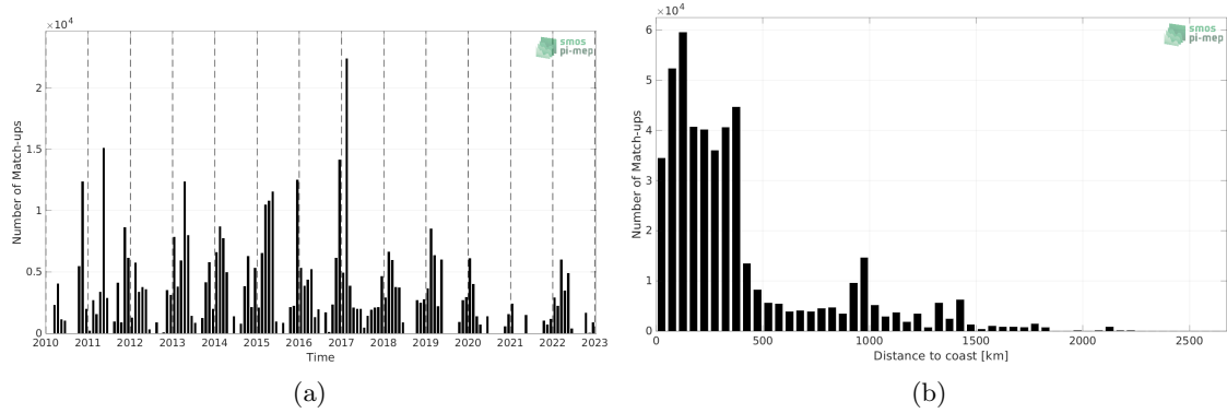
Figure 1: Number of match-ups between TSG (SAMOS) and SMOS SSS L2Q v331 - 0.25 Deg (CATDS-CPDC) SSS as a function of time (a) and as function of the distance to coast (b) over the Southern Ocean Pi-MEP region and for the full satellite product period.
