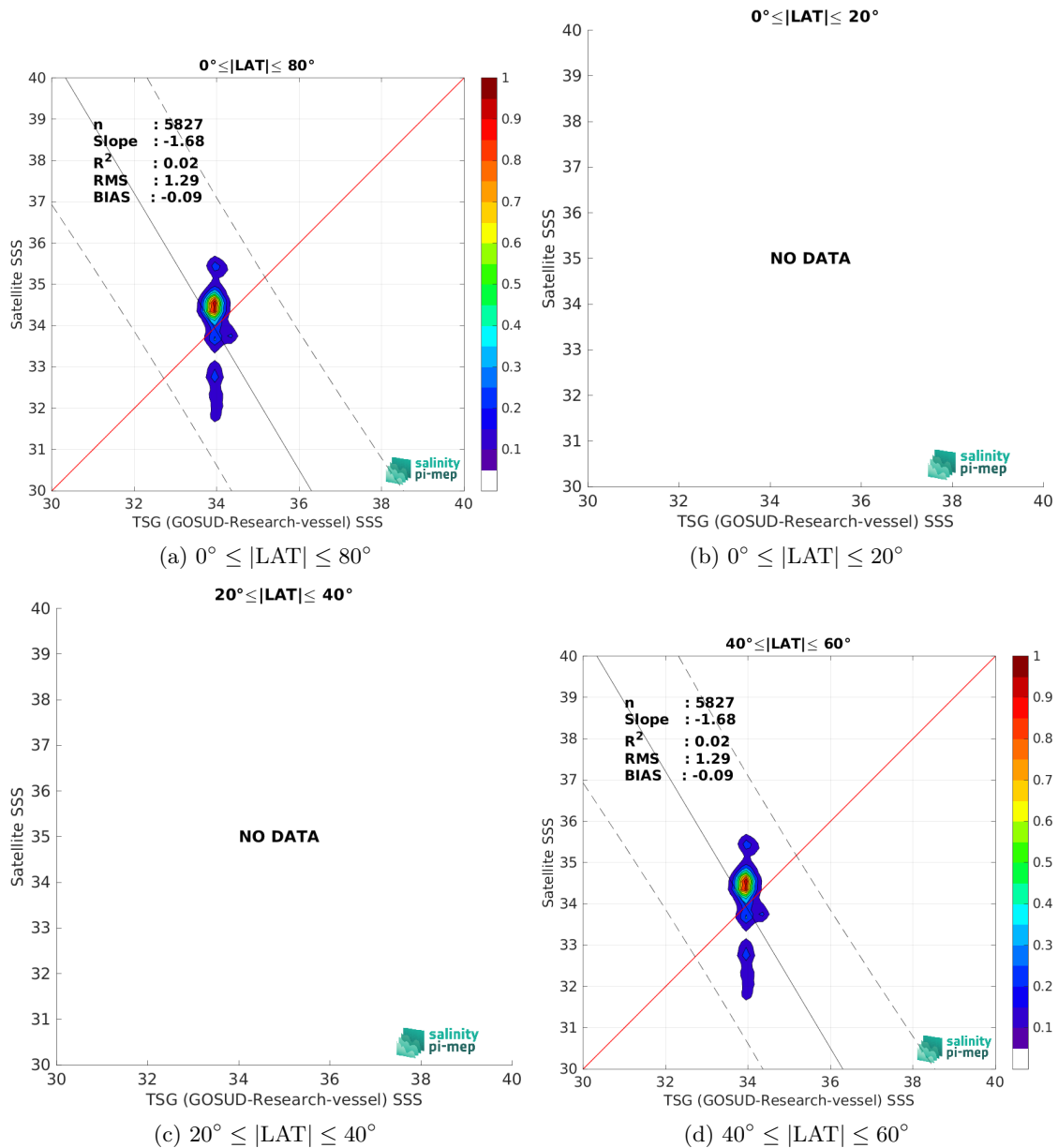
Figure 9: Contour maps of the concentration of SMOS SSS L2Q v331 - 0.25 Deg (CATDS-CPDC) SSS (y-axis) versus TSG (GOSUD-Research-vessel) SSS (x-axis) at match-up pairs for different latitude bands. For each plot, the red line shows x=y . The black thin and dashed lines indicate a linear fit through the data cloud and the \pm 95\% confidence levels, respectively. The number of match-up pairs n , the slope and R^2 coefficient of the linear fit, the root mean square (RMS) and the mean bias between satellite and in situ data are indicated for each latitude band in each plot.
