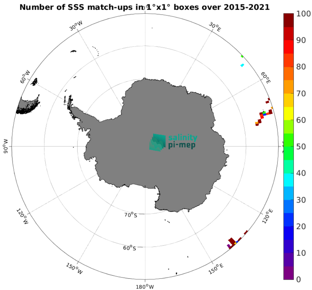
Figure 4: Number of SSS match-ups between TSG (GOSUD-Research-vessel) SSS and the SMOS SSS L2Q v331 - 0.25 Deg (CATDS-CPDC) SSS product for the Southern Ocean Pi-MEP region over 1^{\circ} \times 1^{\circ} boxes and for the full satellite product period.
