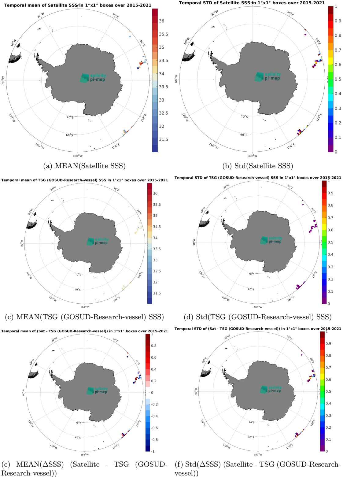
Figure 6: Temporal mean (left) and Std (right) of SSS from SMOS SSS L2Q v331 - 0.25 Deg (CATDS-CPDC) (top), TSG (GOSUD-Research-vessel) (middle), and of \Delta SSS (Satellite - TSG (GOSUD-Research-vessel)). Only match-up pairs are used to generate these maps.
