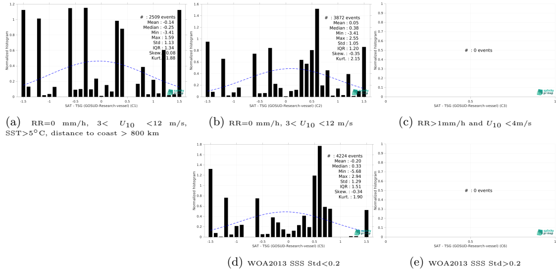
Figure 13: Normalized histogram of \Delta SSS (SMOS SSS L2Q v331 - 0.25 Deg (CATDS-CPDC) - TSG (GOSUD-Research-vessel)) for 5 different subdatasets corresponding to: RR=0 mm/h, 3 < U_{10} < 12 m/s, SST > 5°C, distance to coast > 800 km (a), RR=0 mm/h, 3 < U_{10} < 12 m/s (b), RR > 1mm/h and U_{10} < 4 m/s (c), WOA2013 SSS Std < 0.2 (d), WOA2013 SSS Std > 0.2 (e).
