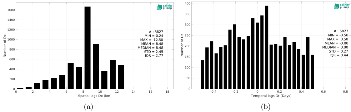
Figure 5: Histograms of the spatial (a) and temporal (b) lags between the location/time of the TSG (GOSUD-Research-vessel) measurement and the date of the corresponding SMOS SSS L2Q v331 - 0.25 Deg (CATDS-CPDC) SSS pixel.
