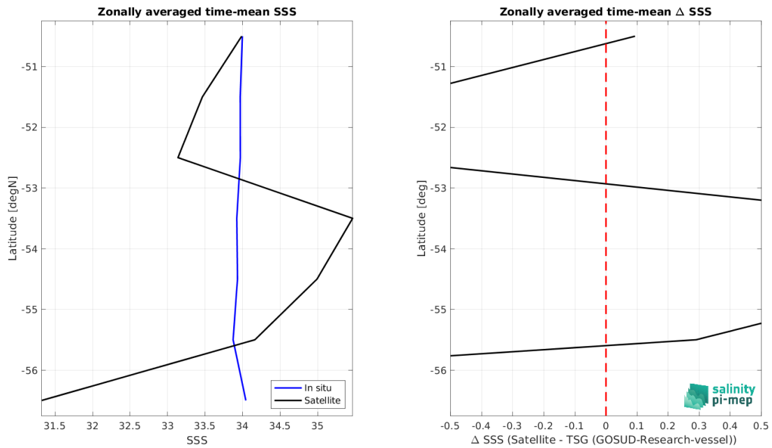
Figure 8: Left panel: Zonal mean SSS from SMOS SSS L2Q v331 - 0.25 Deg (CATDS-CPDC) satellite product (black) and from TSG (GOSUD-Research-vessel) (blue). Right panel: Zonal mean of \Delta SSS (Satellite - TSG (GOSUD-Research-vessel)) for all the collected Pi-MEP match-up pairs estimated over the full satellite product period.
