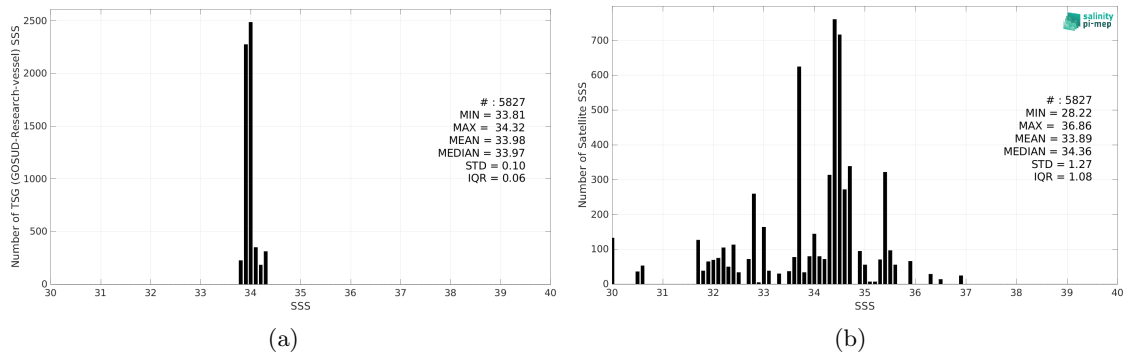
Figure 2: Histograms of SSS from TSG (GOSUD-Research-vessel) (a) and SMOS SSS L2Q v331 - 0.25 Deg (CATDS-CPDC) (b) considering all match-up pairs per bins of 0.1 over the Southern Ocean Pi-MEP region and for the full satellite product period.
