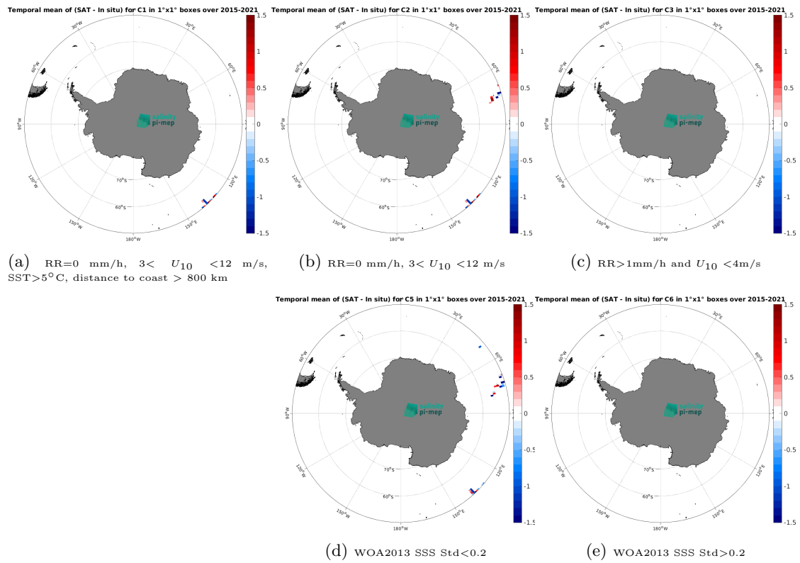
Figure 12: Temporal mean gridded over spatial boxes of size 1^\circ \times 1^\circ of \Delta SSS (SMOS SSS L2Q v331 - 0.25 Deg (CATDS-CPDC) - TSG (GOSUD-Research-vessel)) for 5 different subdatasets corresponding to:RR=0 mm/h, 3 < U_{10} < 12 m/s, SST>5°C, distance to coast > 800 km (a), RR=0 mm/h, 3 < U_{10} < 12 m/s (b), RR>1mm/h and U_{10} < 4 m/s (c), WOA2013 SSS Std<0.2 (d), WOA2013 SSS Std>0.2 (e).
