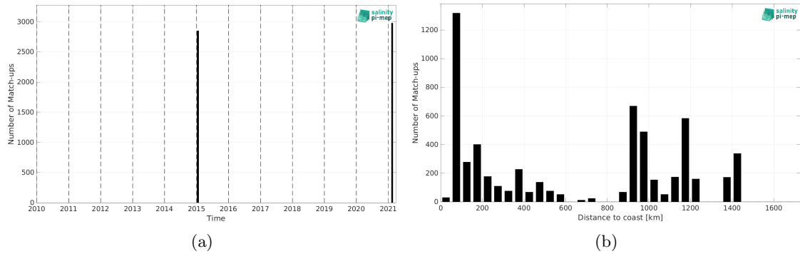
Figure 1: Number of match-ups between TSG (GOSUD-Research-vessel) and SMOS SSS L2Q v331 - 0.25 Deg (CATDS-CPDC) SSS as a function of time (a) and as function of the distance to coast (b) over the Southern Ocean Pi-MEP region and for the full satellite product period.
