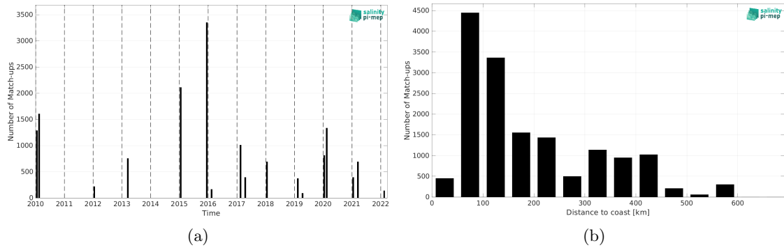
Figure 1: Number of match-ups between TSG (CSIC-UTM) and SMOS SSS L2Q v331 - 0.25 Deg (CATDS-CPDC) SSS as a function of time (a) and as function of the distance to coast (b) over the Southern Ocean Pi-MEP region and for the full satellite product period.
