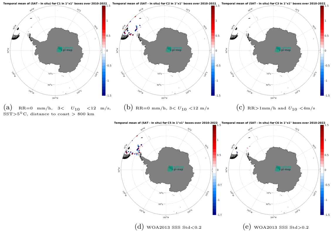
Figure 12: Temporal mean gridded over spatial boxes of size 1^{\circ}\times 1^{\circ} of \Delta\text{SSS} (SMOS SSS L2Q v331 - 0.25 Deg (CATDS-CPDC) - TSG (CSIC-UTM)) for 5 different subdatasets corresponding to: RR=0 mm/h, 3 < U_{10} < 12 m/s, SST >5^{\circ}\text{C} , distance to coast > 800 km (a), RR=0 mm/h, 3 < U_{10} < 12 m/s (b), RR >1 mm/h and U_{10} < 4 m/s (c), WOA2013 SSS Std <0.2 (d), WOA2013 SSS Std >0.2 (e).
