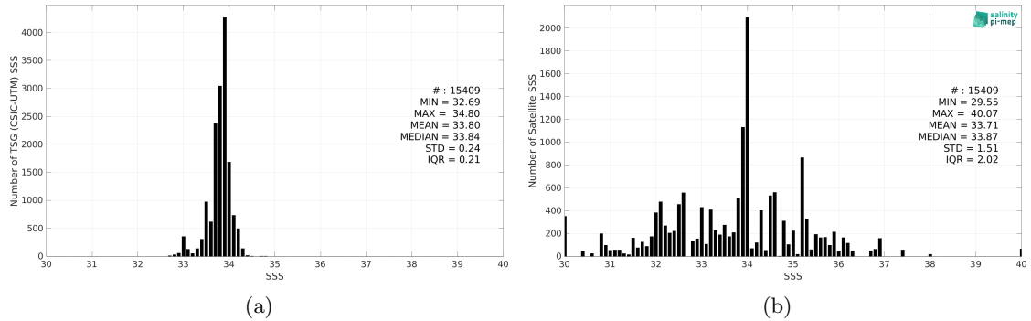
Figure 2: Histograms of SSS from TSG (CSIC-UTM) (a) and SMOS SSS L2Q v331 - 0.25 Deg (CATDS-CPDC) (b) considering all match-up pairs per bins of 0.1 over the Southern Ocean Pi-MEP region and for the full satellite product period.
