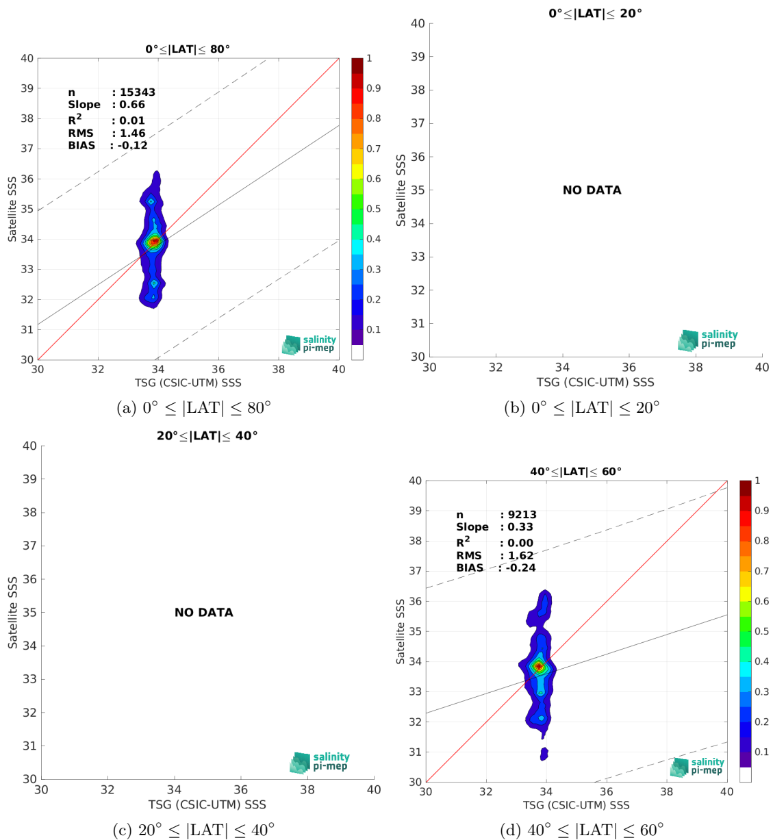
Figure 9: Contour maps of the concentration of SMOS SSS L2Q v331 - 0.25 Deg (CATDS-CPDC) SSS (y-axis) versus TSG (CSIC-UTM) SSS (x-axis) at match-up pairs for different latitude bands. For each plot, the red line shows x=y . The black thin and dashed lines indicate a linear fit through the data cloud and the \pm 95\% confidence levels, respectively. The number match-up pairs n , the slope and R^2 coefficient of the linear fit, the root mean square (RMS) and the mean bias between satellite and in situ data are indicated for each latitude band in each plots.
