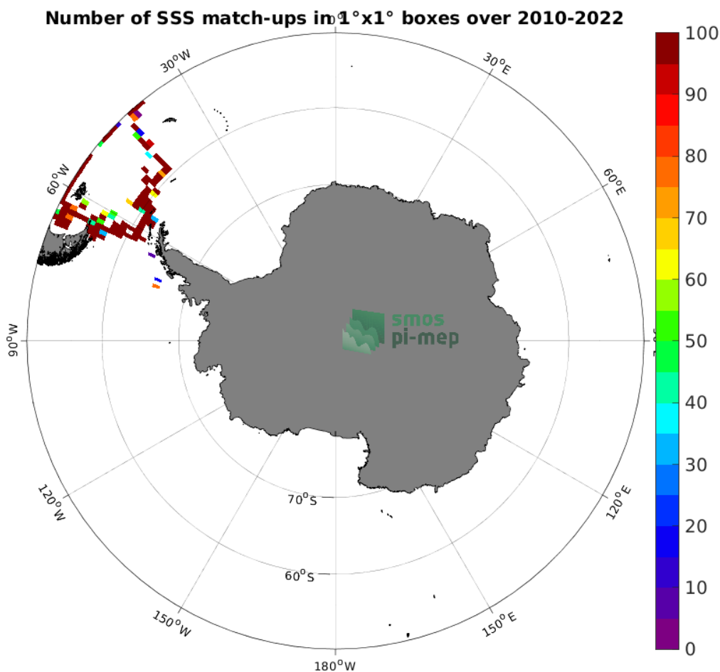
Figure 4: Number of SSS match-ups between TSG (CSIC-UTM) SSS and the SMOS SSS L2Q v331 - 0.25 Deg (CATDS-CPDC) SSS product for the Southern Ocean Pi-MEP region over 1^\circ \times 1^\circ boxes and for the full satellite product period.
