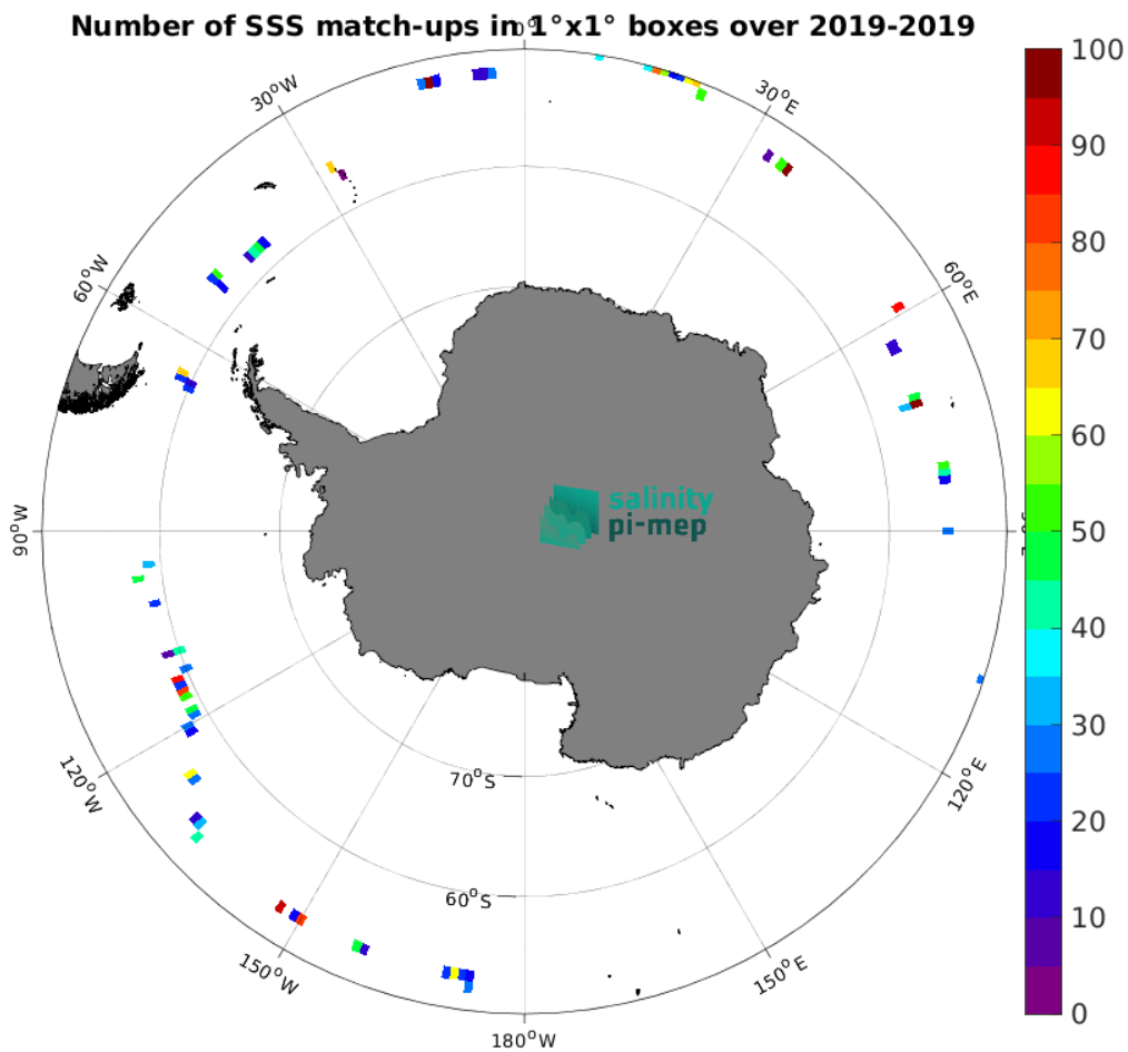
Figure 4: Number of SSS match-ups between Saildrone SSS and the SMOS SSS L2Q v331 - 0.25 Deg (CATDS-CPDC) SSS product for the Southern Ocean Pi-MEP region over 1^{\circ} \times 1^{\circ} boxes and for the full satellite product period.
