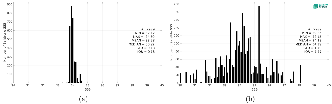
Figure 2: Histograms of SSS from Saildrone (a) and SMOS SSS L2Q v331 - 0.25 Deg (CATDS-CPDC) (b) considering all match-up pairs per bins of 0.1 over the Southern Ocean Pi-MEP region and for the full satellite product period.
