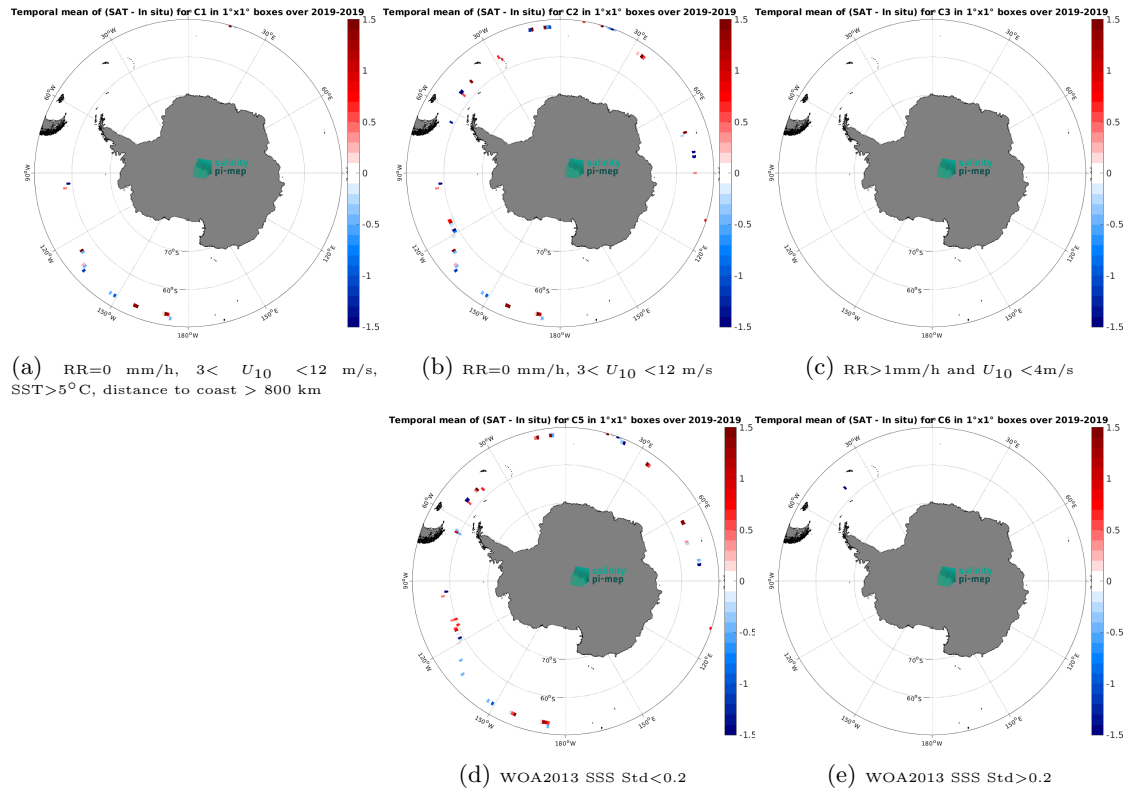
Figure 12: Temporal mean gridded over spatial boxes of size 1^{\circ}\times 1^{\circ} of \Delta\text{SSS} (SMOS SSS L2Q v331 - 0.25 Deg (CATDS-CPDC) - Saildrone) for 5 different subdatasets corresponding to:RR=0 mm/h, 3 < U_{10} < 12 m/s, SST >5^{\circ}\text{C} , distance to coast > 800 km (a), RR=0 mm/h, 3 < U_{10} < 12 m/s (b), RR >1 mm/h and U_{10} < 4 m/s (c), WOA2013 SSS Std <0.2 (d), WOA2013 SSS Std >0.2 (e).
