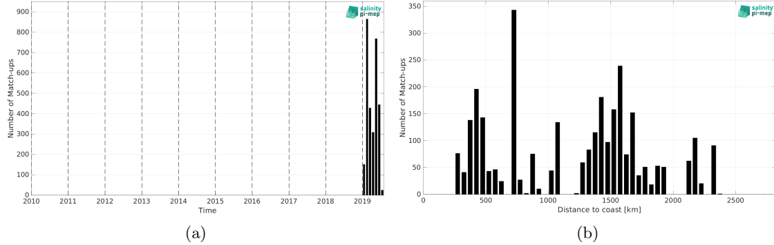
Figure 1: Number of match-ups between Saildrone and SMOS SSS L2Q v331 - 0.25 Deg (CATDS-CPDC) SSS as a function of time (a) and as function of the distance to coast (b) over the Southern Ocean Pi-MEP region and for the full satellite product period.
