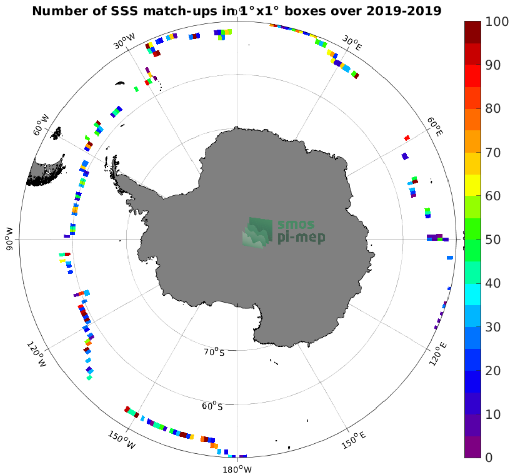
Figure 4: Number of SSS match-ups between Sairdrone SSS and the SMOS SSS L2Q v331 - 0.25 Deg (CATDS-CPDC) SSS product for the Southern Ocean Pi-MEP region over 1^\circ \times 1^\circ boxes and for the full satellite product period.
