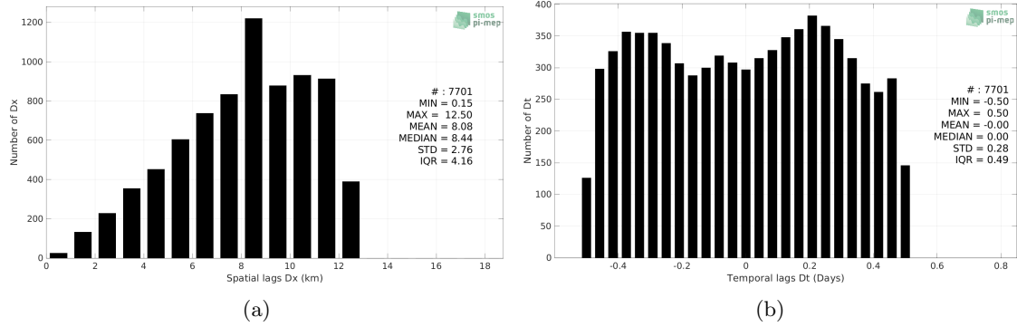
Figure 5: Histograms of the spatial (a) and temporal (b) lags between the location/time of the Sairdron measurement and the date of the corresponding SMOS SSS L2Q v331 - 0.25 Deg (CATDS-CPDC) SSS pixel.
