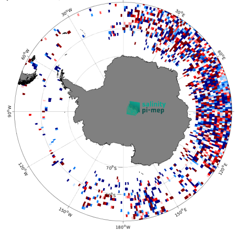
(e) MEAN( \Delta SSS) (Satellite - Marine mammals) 16
