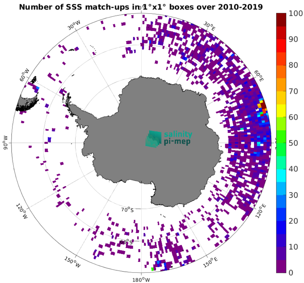
Figure 4: Number of SSS match-ups between Marine mammals SSS and the SMOS SSS L2Q v331 - 0.25 Deg (CATDS-CPDC) SSS product for the Southern Ocean Pi-MEP region over 1^{\circ} \times 1^{\circ} boxes and for the full satellite product period.
