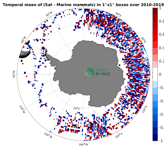
(e) MEAN( \Delta SSS) (Satellite - Marine mammals) 16
