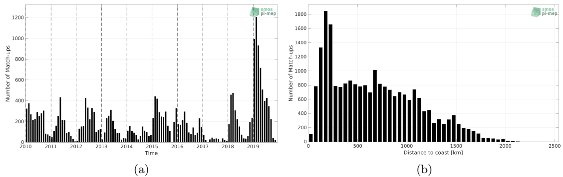
Figure 1: Number of match-ups between Marine mammals and SMOS SSS L2Q v331 - 0.25 Deg (CATDS-CPDC) SSS as a function of time (a) and as function of the distance to coast (b) over the Southern Ocean Pi-MEP region and for the full satellite product period.
