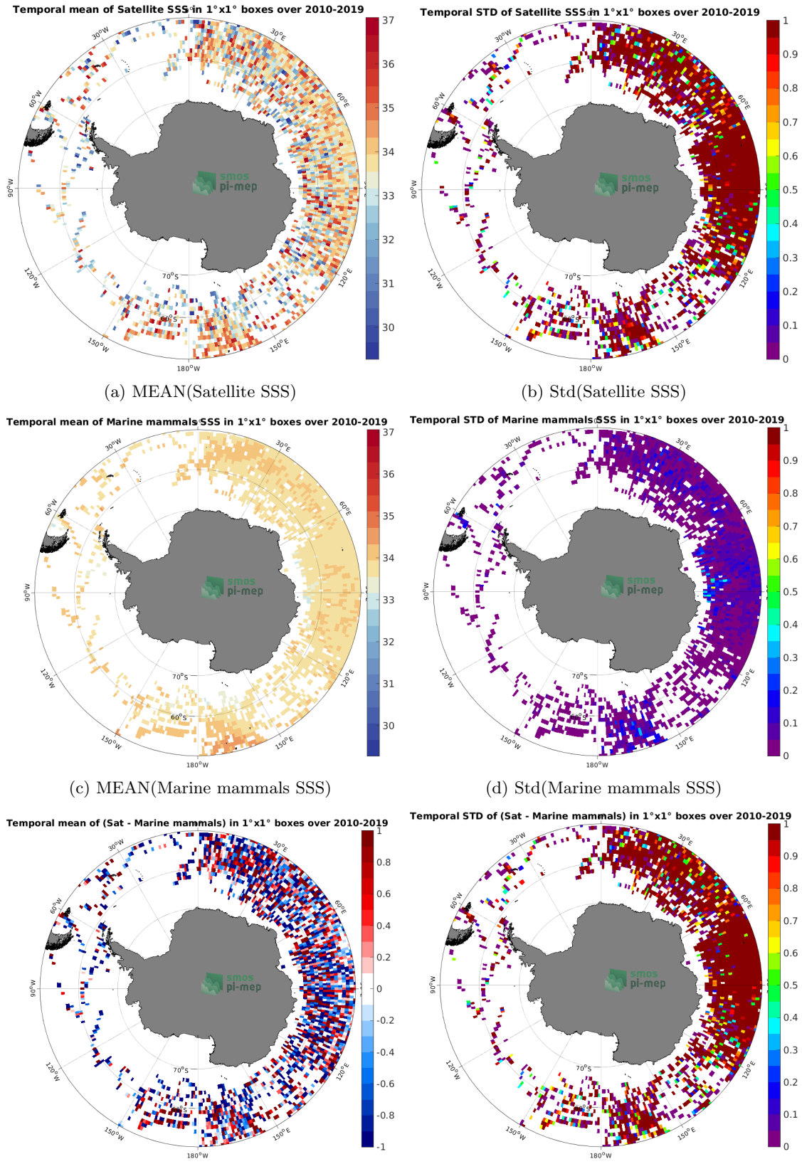
(e) MEAN( \Delta SSS) (Satellite - Marine mammals) 16
