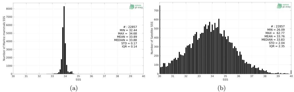
Figure 2: Histograms of SSS from Marine mammals (a) and SMOS SSS L2Q v331 - 0.25 Deg (CATDS-CPDC) (b) considering all match-up pairs per bins of 0.1 over the Southern Ocean Pi-MEP region and for the full satellite product period.
