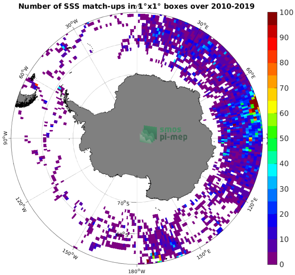
Figure 4: Number of SSS match-ups between Marine mammals SSS and the SMOS SSS L2Q v331 - 0.25 Deg (CATDS-CPDC) SSS product for the Southern Ocean Pi-MEP region over 1^\circ \times 1^\circ boxes and for the full satellite product period.
