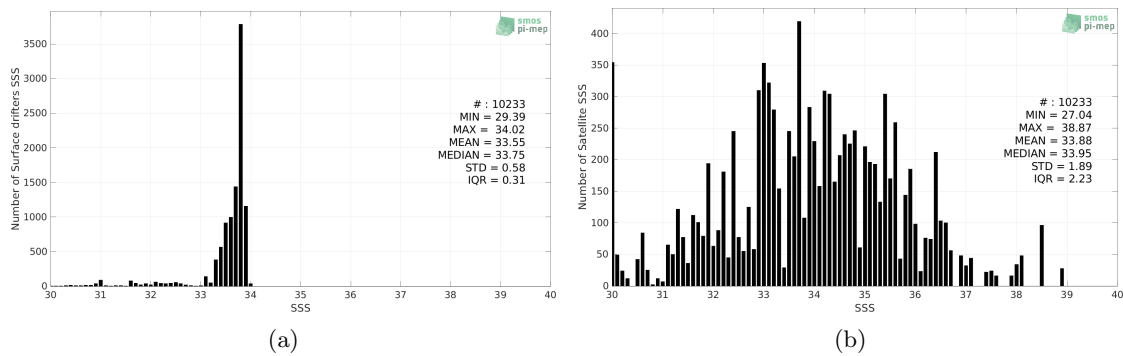
Figure 2: Histograms of SSS from Surface drifters (a) and SMOS SSS L2Q v331 - 0.25 Deg (CATDS-CPDC) (b) considering all match-up pairs per bins of 0.1 over the Southern Ocean Pi-MEP region and for the full satellite product period.
