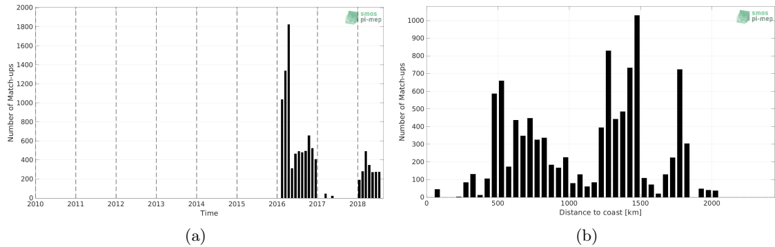
Figure 1: Number of match-ups between Surface drifters and SMOS SSS L2Q v331 - 0.25 Deg (CATDS-CPDC) SSS as a function of time (a) and as function of the distance to coast (b) over the Southern Ocean Pi-MEP region and for the full satellite product period.
