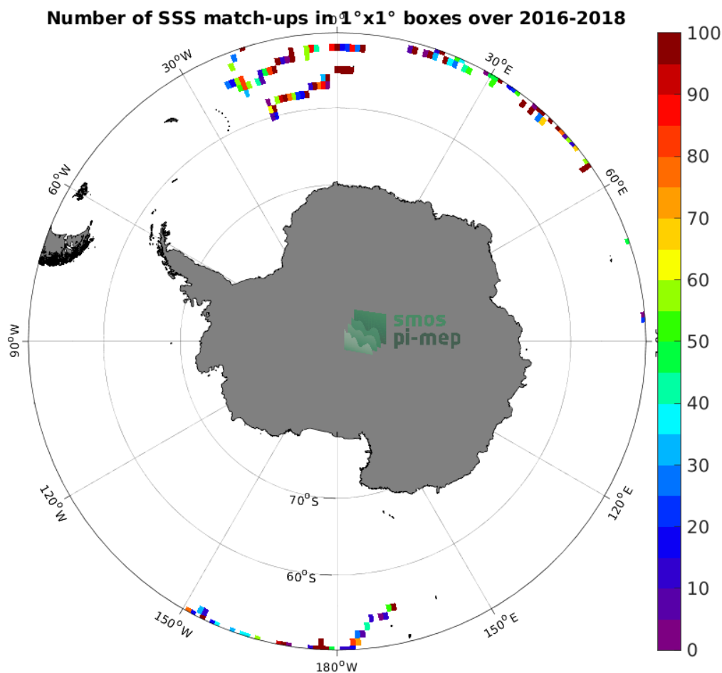
Figure 3: Number of SSS match-ups between Surface drifters SSS and the SMOS SSS L2Q v331 - 0.25 Deg (CATDS-CPDC) SSS product for the Southern Ocean Pi-MEP region over 1^\circ \times 1^\circ boxes and for the full satellite product period.
