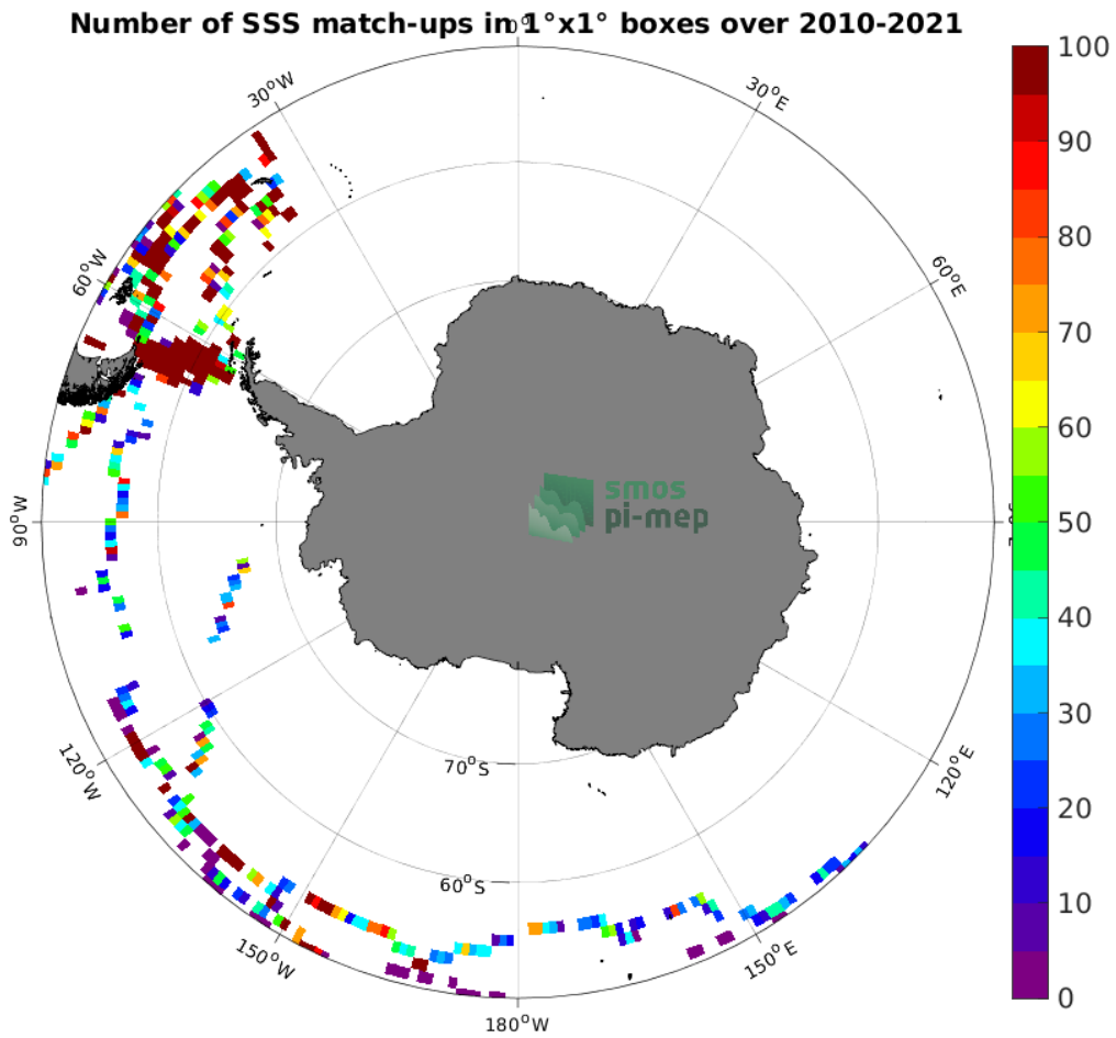
Figure 4: Number of SSS match-ups between TSG (GOSUD-Sailing-ship) SSS and the SMOS SSS L2Q v330 - 0.25 Deg (CATDS-CPDC) SSS product for the Southern Ocean Pi-MEP region over 1°x1° boxes and for the full satellite product period.
