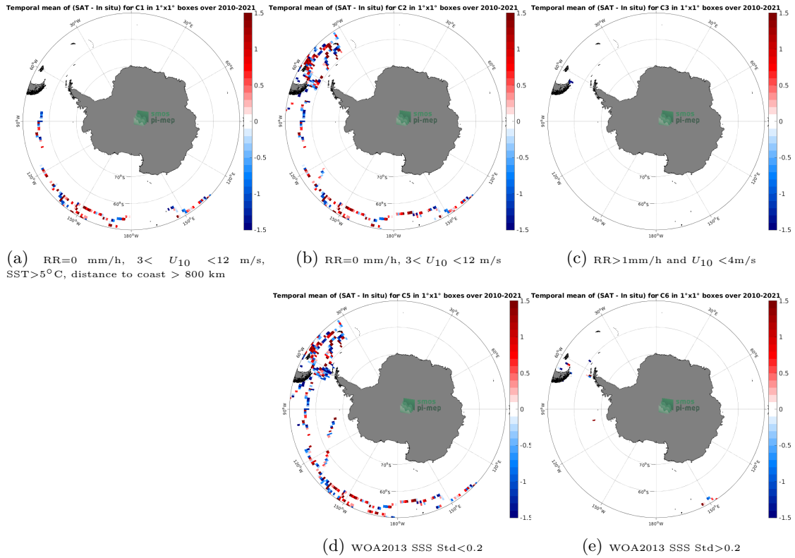
Figure 12: Temporal mean gridded over spatial boxes of size 1^{\circ} \times 1^{\circ} of \Delta SSS (SMOS SSS L2Q v330 - 0.25 Deg (CATDS-CPDC) - TSG (GOSUD-Sailing-ship)) for 5 different subdatasets corresponding to: RR=0 mm/h, 3 < U_{10} < 12 m/s, SST>5°C, distance to coast > 800 km (a), RR=0 mm/h, 3 < U_{10} < 12 m/s (b), RR>1mm/h and U_{10} < 4 m/s (c), WOA2013 SSS Std<0.2 (d), WOA2013 SSS Std>0.2 (e).
