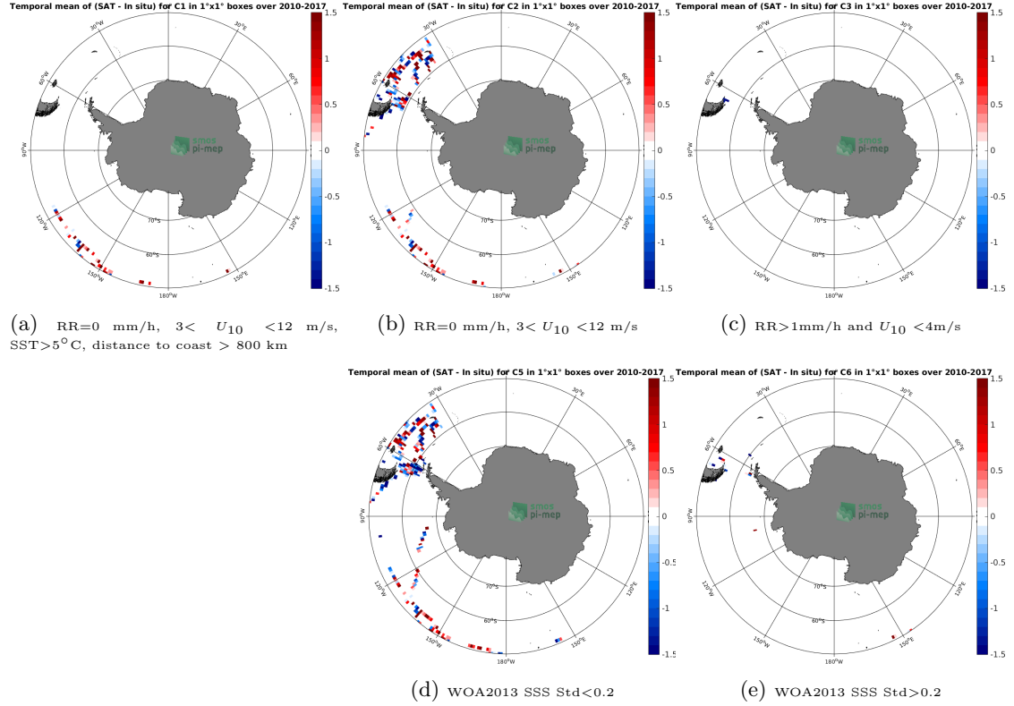
Figure 12: Temporal mean gridded over spatial boxes of size 1°×1° of \Delta SSS (SMOS SSS L2Q v330 - 0.25 Deg (CATDS-CPDC) - TSG (GOSUD-Sailing-ship)) for 5 different subdatasets corresponding to:RR=0 mm/h, 3 < U_{10} < 12 m/s, SST>5°C, distance to coast > 800 km (a), RR=0 mm/h, 3 < U_{10} < 12 m/s (b), RR>1mm/h and U_{10} < 4 m/s (c), WOA2013 SSS Std<0.2 (d), WOA2013 SSS Std>0.2 (e).
