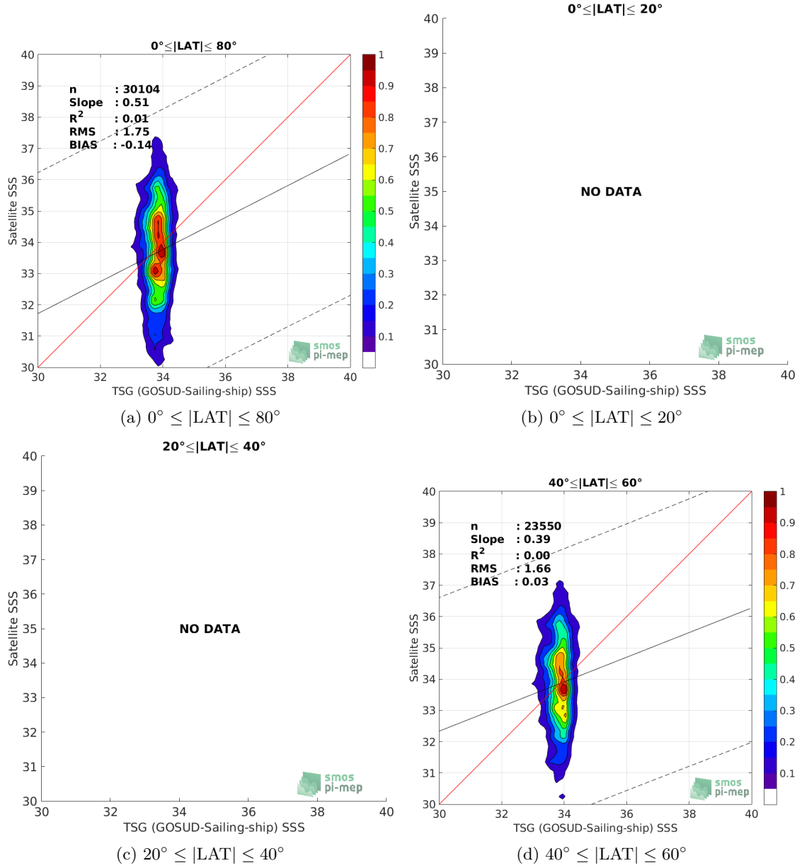
Figure 9: Contour maps of the concentration of SMOS SSS L2Q v330 - 0.25 Deg (CATDS-CPDC) SSS (y-axis) versus TSG (GOSUD-Sailing-ship) SSS (x-axis) at match-up pairs for different latitude bands. For each plot, the red line shows x=y . The black thin and dashed lines indicate a linear fit through the data cloud and the \pm 95\% confidence levels, respectively. The number match-up pairs n , the slope and R^2 coefficient of the linear fit, the root mean square (RMS) and the mean bias between satellite and in situ data are indicated for each latitude band in each plots.
