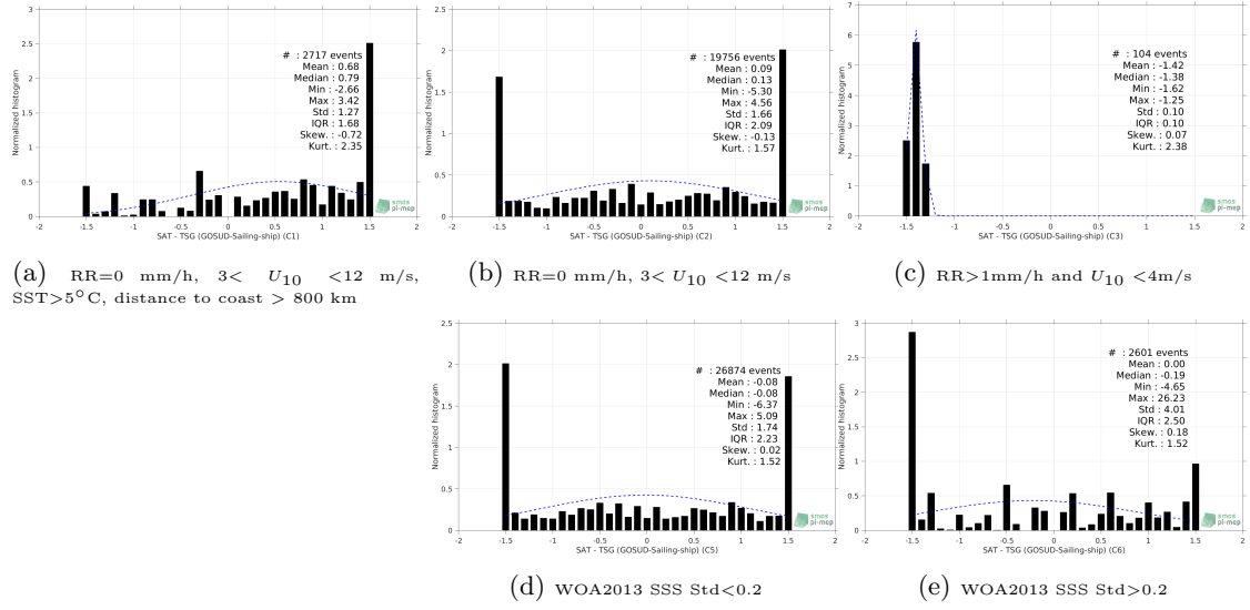
Figure 13: Normalized histogram of \Delta\text{SSS} (SMOS SSS L2Q v330 - 0.25 Deg (CATDS-CPDC) - TSG (GOSUD-Sailing-ship)) for 5 different subdatasets corresponding to: RR=0 mm/h, 3 < U_{10} < 12 m/s, SST > 5^\circ\text{C} , distance to coast > 800 km (a), RR=0 mm/h, 3 < U_{10} < 12 m/s (b), RR > 1\text{mm/h} and U_{10} < 4\text{m/s} (c), WOA2013 SSS Std < 0.2 (d), WOA2013 SSS Std > 0.2 (e).
