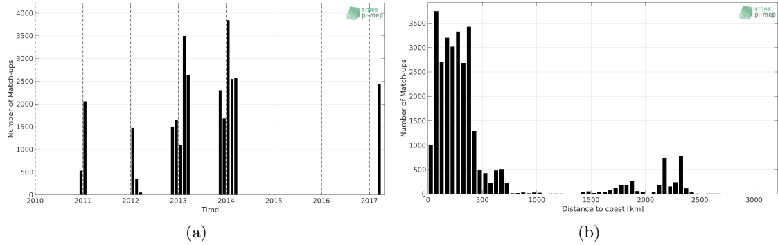
Figure 1: Number of match-ups between TSG (GOSUD-Sailing-ship) and SMOS SSS L2Q v330 - 0.25 Deg (CATDS-CPDC) SSS as a function of time (a) and as function of the distance to coast (b) over the Southern Ocean Pi-MEP region and for the full satellite product period.
