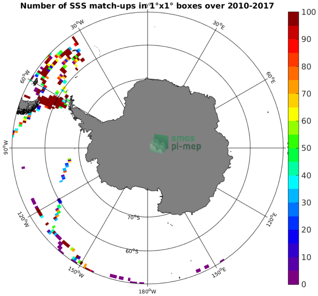
Figure 4: Number of SSS match-ups between TSG (GOSUD-Sailing-ship) SSS and the SMOS SSS L2Q v330 - 0.25 Deg (CATDS-CPDC) SSS product for the Southern Ocean Pi-MEP region over 1^\circ \times 1^\circ boxes and for the full satellite product period.
