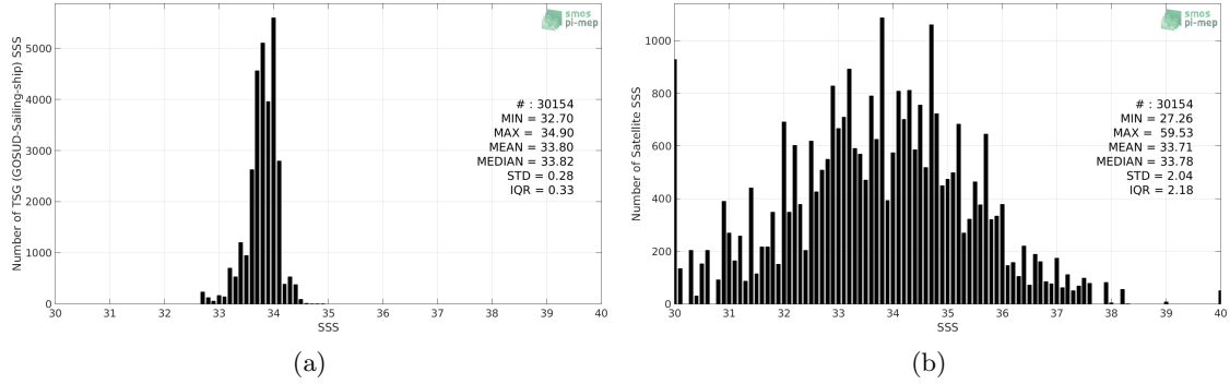
Figure 2: Histograms of SSS from TSG (GOSUD-Sailing-ship) (a) and SMOS SSS L2Q v330 - 0.25 Deg (CATDS-CPDC) (b) considering all match-up pairs per bins of 0.1 over the Southern Ocean Pi-MEP region and for the full satellite product period.
