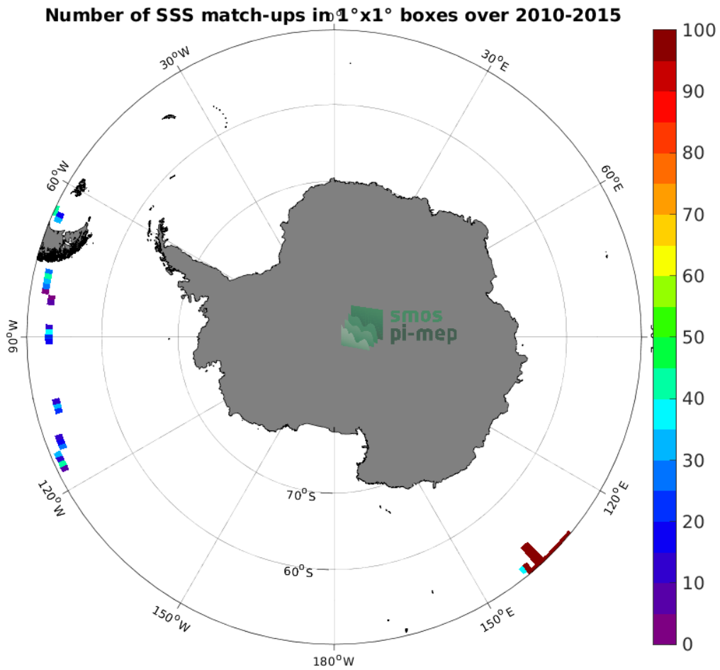
Figure 4: Number of SSS match-ups between TSG (GOSUD-Research-vessel) SSS and the SMOS SSS L2Q v330 - 0.25 Deg (CATDS-CPDC) SSS product for the Southern Ocean Pi-MEP region over 1°x1° boxes and for the full satellite product period.
