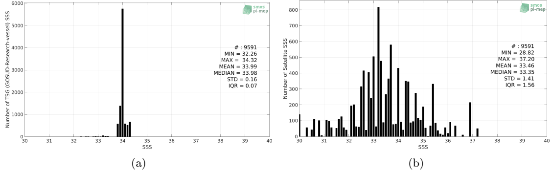
Figure 2: Histograms of SSS from TSG (GOSUD-Research-vessel) (a) and SMOS SSS L2Q v330 - 0.25 Deg (CATDS-CPDC) (b) considering all match-up pairs per bins of 0.1 over the Southern Ocean Pi-MEP region and for the full satellite product period.
