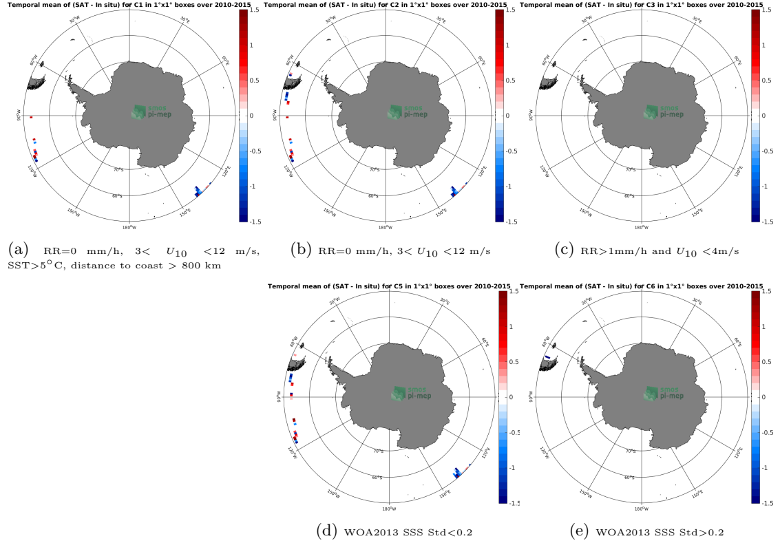
Figure 12: Temporal mean gridded over spatial boxes of size 1^{\circ} \times 1^{\circ} of \Delta\text{SSS} (SMOS SSS L2Q v330 - 0.25 Deg (CATDS-CPDC) - TSG (GOSUD-Research-vessel)) for 5 different subdatasets corresponding to: RR=0 mm/h, 3 < U_{10} < 12 m/s, SST > 5^{\circ}\text{C} , distance to coast > 800 km (a), RR=0 mm/h, 3 < U_{10} < 12 m/s (b), RR > 1 mm/h and U_{10} < 4 m/s (c), WOA2013 SSS Std < 0.2 (d), WOA2013 SSS Std > 0.2 (e).
