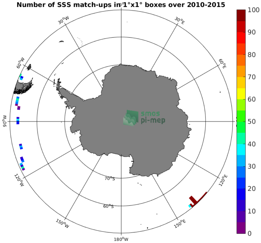
Figure 4: Number of SSS match-ups between TSG (GOSUD-Research-vessel) SSS and the SMOS SSS L2Q v330 - 0.25 Deg (CATDS-CPDC) SSS product for the Southern Ocean Pi-MEP region over 1^\circ \times 1^\circ boxes and for the full satellite product period.
