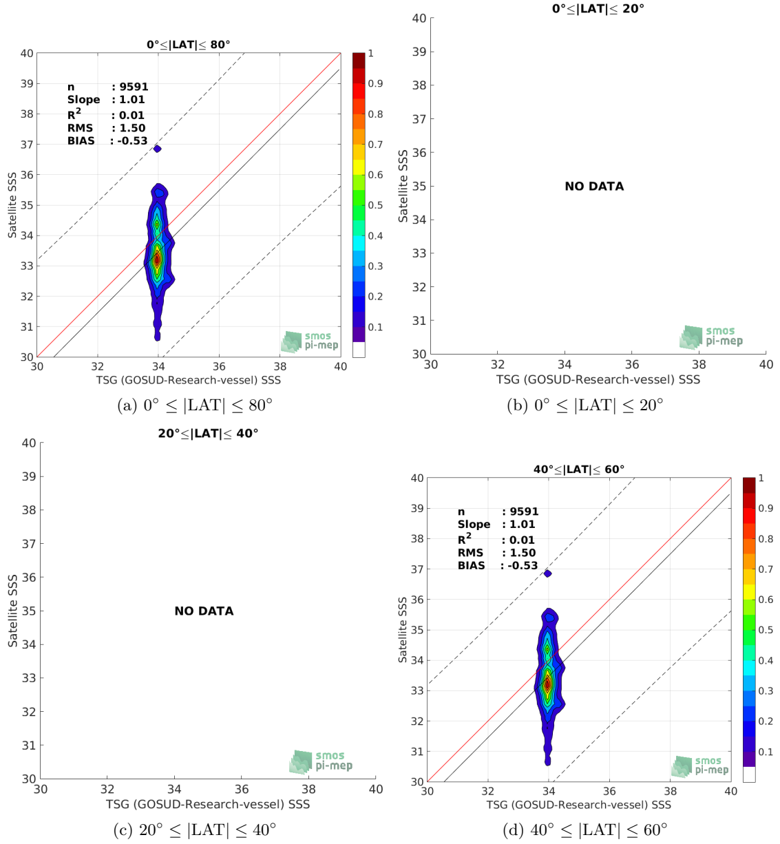
Figure 9: Contour maps of the concentration of SMOS SSS L2Q v330 - 0.25 Deg (CATDS-CPDC) SSS (y-axis) versus TSG (GOSUD-Research-vessel) SSS (x-axis) at match-up pairs for different latitude bands. For each plot, the red line shows x=y . The black thin and dashed lines indicate a linear fit through the data cloud and the \pm 95\% confidence levels, respectively. The number match-up pairs n , the slope and R^2 coefficient of the linear fit, the root mean square (RMS) and the mean bias between satellite and in situ data are indicated for each latitude band in each plots.
