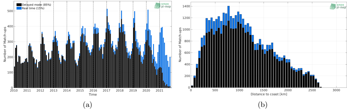
Figure 1: Number of match-ups between Argo and SMOS SSS L2Q v330 - 0.25 Deg (CATDS-CPDC) SSS as a function of time (a) and as function of the distance to coast (b) over the Southern Ocean Pi-MEP region and for the full satellite product period.
