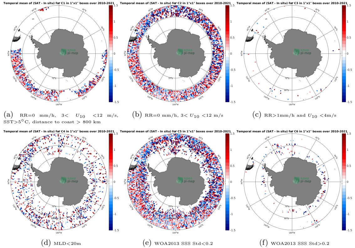
Figure 12: Temporal mean gridded over spatial boxes of size 1^{\circ} \times 1^{\circ} of \Delta\text{SSS} (SMOS SSS L2Q v330 - 0.25 Deg (CATDS-CPDC) - Argo) for 6 different subdatasets corresponding to: RR=0 mm/h, 3 < U_{10} < 12 m/s, SST >5^{\circ}\text{C} , distance to coast > 800 km (a), RR=0 mm/h, 3 < U_{10} < 12 m/s (b), RR >1 mm/h and U_{10} < 4 m/s (c),MLD <20 m (d),WOA2013 SSS Std <0.2 (e),WOA2013 SSS Std >0.2 (f).
