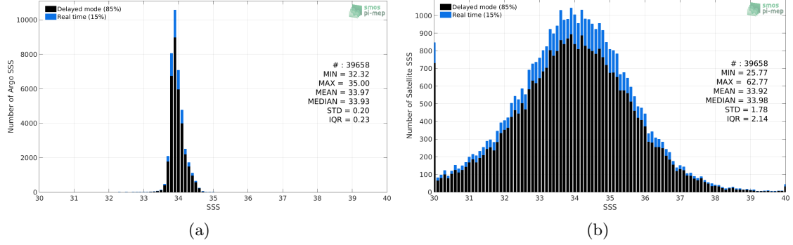
Figure 2: Histograms of SSS from Argo (a) and SMOS SSS L2Q v330 - 0.25 Deg (CATDS-CPDC) (b) considering all match-up pairs per bins of 0.1 over the Southern Ocean Pi-MEP region and for the full satellite product period.
