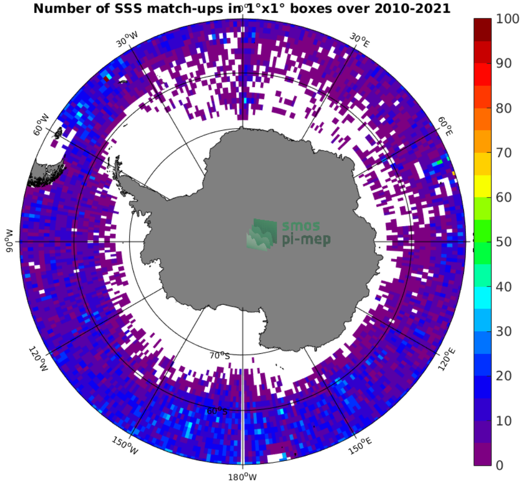
Figure 4: Number of SSS match-ups between Argo SSS and the SMOS SSS L2Q v330 - 0.25 Deg (CATDS-CPDC) SSS product for the Southern Ocean Pi-MEP region over 1^\circ \times 1^\circ boxes and for the full satellite product period.
