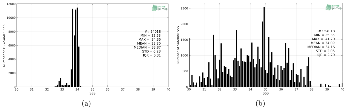
Figure 2: Histograms of SSS from TSG-SAMOS (a) and SMOS-L3-CATDS-CPDC-V321-L2Q (b) considering all match-up pairs per bins of 0.1 over the Southern Ocean Pi-MEP region and for the full satellite product period.
