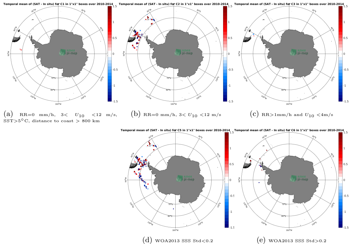
Figure 12: Temporal mean gridded over spatial boxes of size 1^\circ \times 1^\circ of \Delta SSS (SMOS-L3-CATDS-CPDC-V321-L2Q - TSG-SAMOS) for 5 different subdatasets corresponding to:RR=0 mm/h, 3 < U_{10} < 12 m/s, SST >5^\circ\text{C} , distance to coast > 800 km (a), RR=0 mm/h, 3 < U_{10} < 12 m/s (b), RR >1 mm/h and U_{10} < 4 m/s (c), WOA2013 SSS Std <0.2 (d), WOA2013 SSS Std >0.2 (e).
