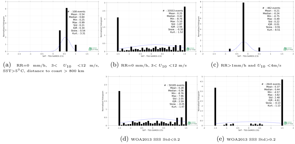
Figure 13: Normalized histogram of \Delta SSS (SMOS-L3-CATDS-CPDC-V321-L2Q - TSG-SAMOS) for 5 different subdatasets corresponding to: RR=0 mm/h, 3 < U_{10} < 12 m/s, SST>5°C, distance to coast > 800 km (a), RR=0 mm/h, 3 < U_{10} < 12 m/s (b), RR>1mm/h and U_{10} < 4 m/s (c), WOA2013 SSS Std<0.2 (d), WOA2013 SSS Std>0.2 (e).
