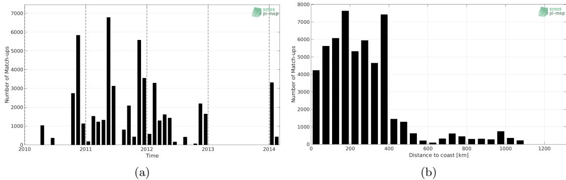
Figure 1: Number of match-ups between TSG-SAMOS and SMOS-L3-CATDS-CPDC-V321-L2Q SSS as a function of time (a) and as function of the distance to coast (b) over the Southern Ocean Pi-MEP region and for the full satellite product period.
