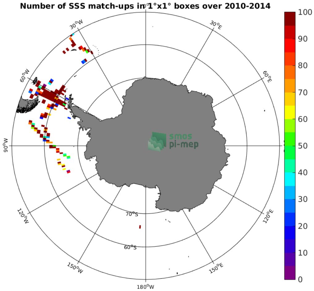
Figure 4: Number of SSS match-ups between TSG-SAMOS SSS and the SMOS-L3-CATDS-CPDC-V321-L2Q SSS product for the Southern Ocean Pi-MEP region over 1°x1° boxes and for the full satellite product period.
