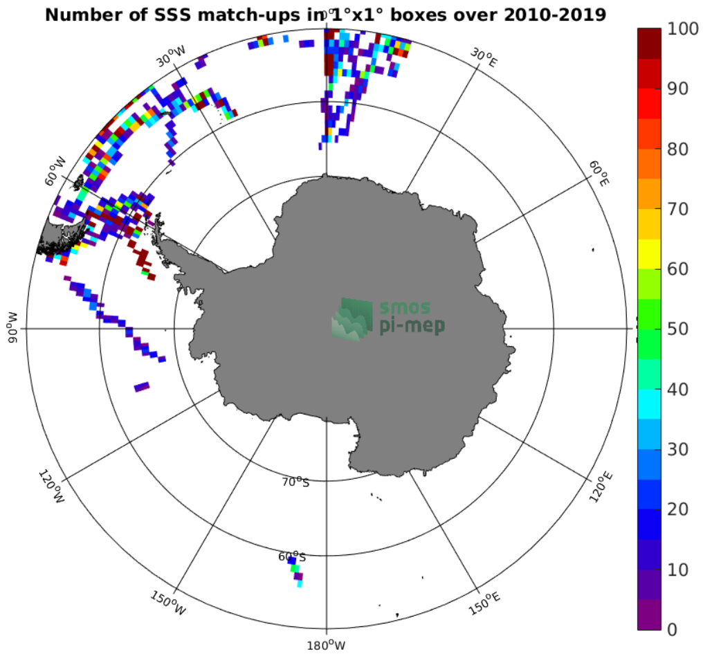
Figure 4: Number of SSS match-ups between TSG (Polarstern) SSS and the SMOS SSS L2Q v321 - 0.25 Deg (CATDS-CPDC) SSS product for the Southern Ocean Pi-MEP region over 1^\circ \times 1^\circ boxes and for the full satellite product period.
